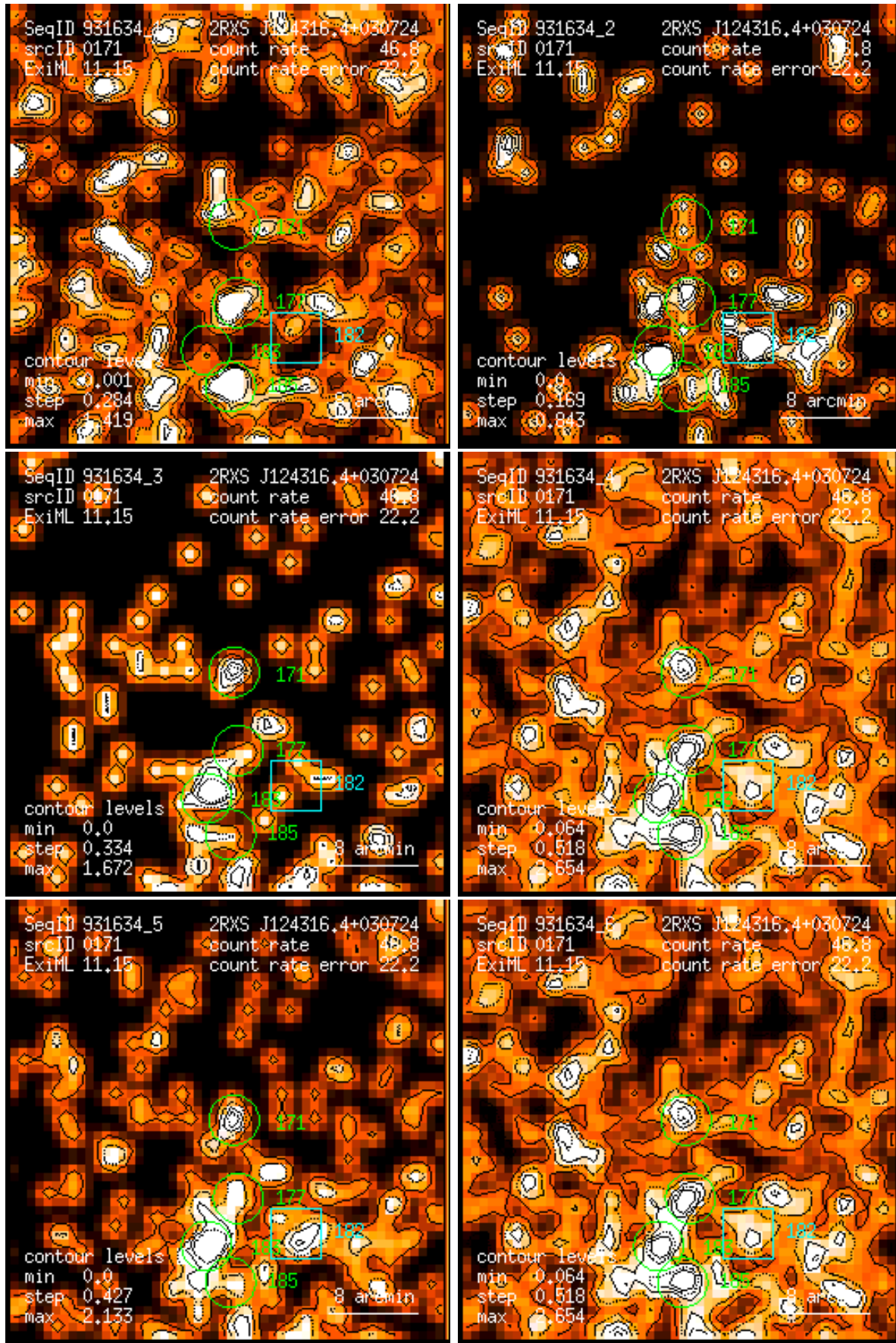
Figure 171: RASS 931634: detection 0171: band rate images, Gaussian filter: (1) PSPC channels 11 – 41, (2) 52 – 90, (3) 91 – 201, (4) 11 – 235, (5) 52 – 201, (6) 11 – 201. Broad band rates in counts/ks. Band rate contour levels in counts/ks/arcmin 2 .
