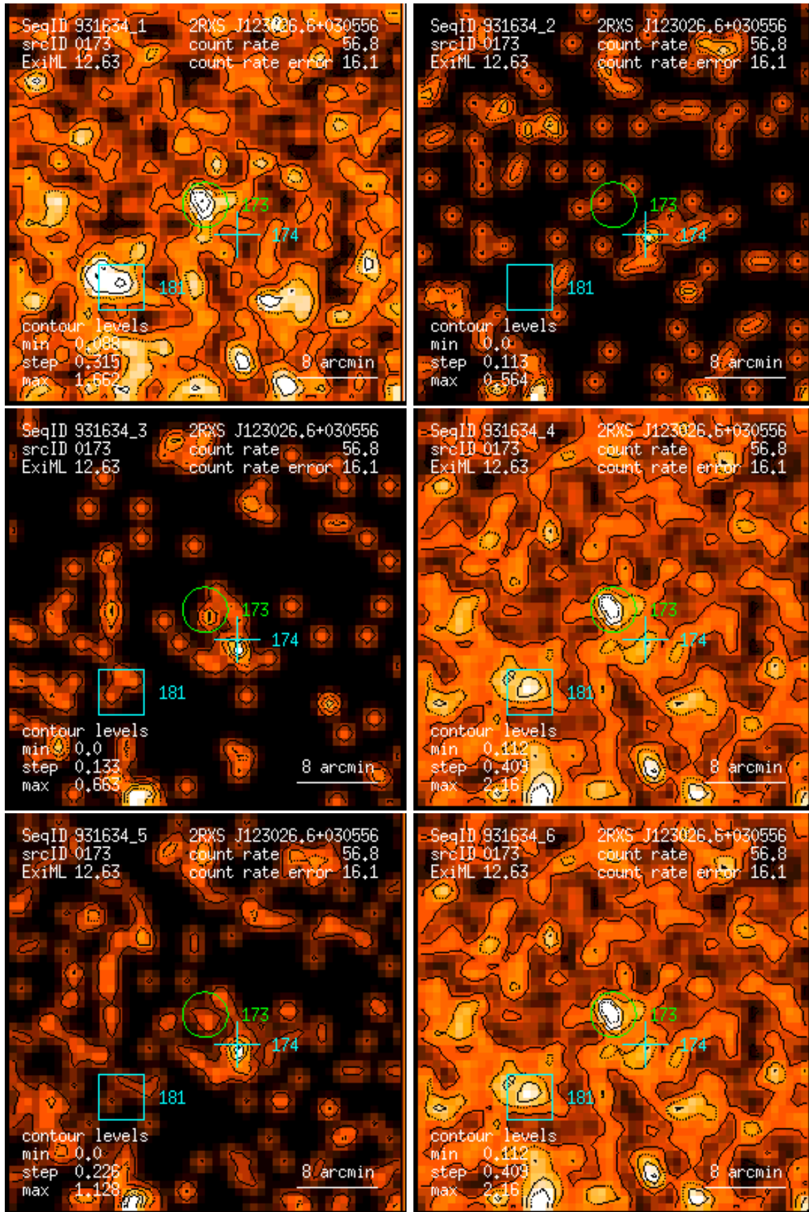
Figure 173: RASS 931634: detection 0173: band rate images, Gaussian filter: (1) PSPC channels 11 – 41, (2) 52 – 90, (3) 91 – 201, (4) 11 – 235, (5) 52 – 201, (6) 11 – 201. Broad band rates in counts/ks. Band rate contour levels in counts/ks/arcmin 2 .
