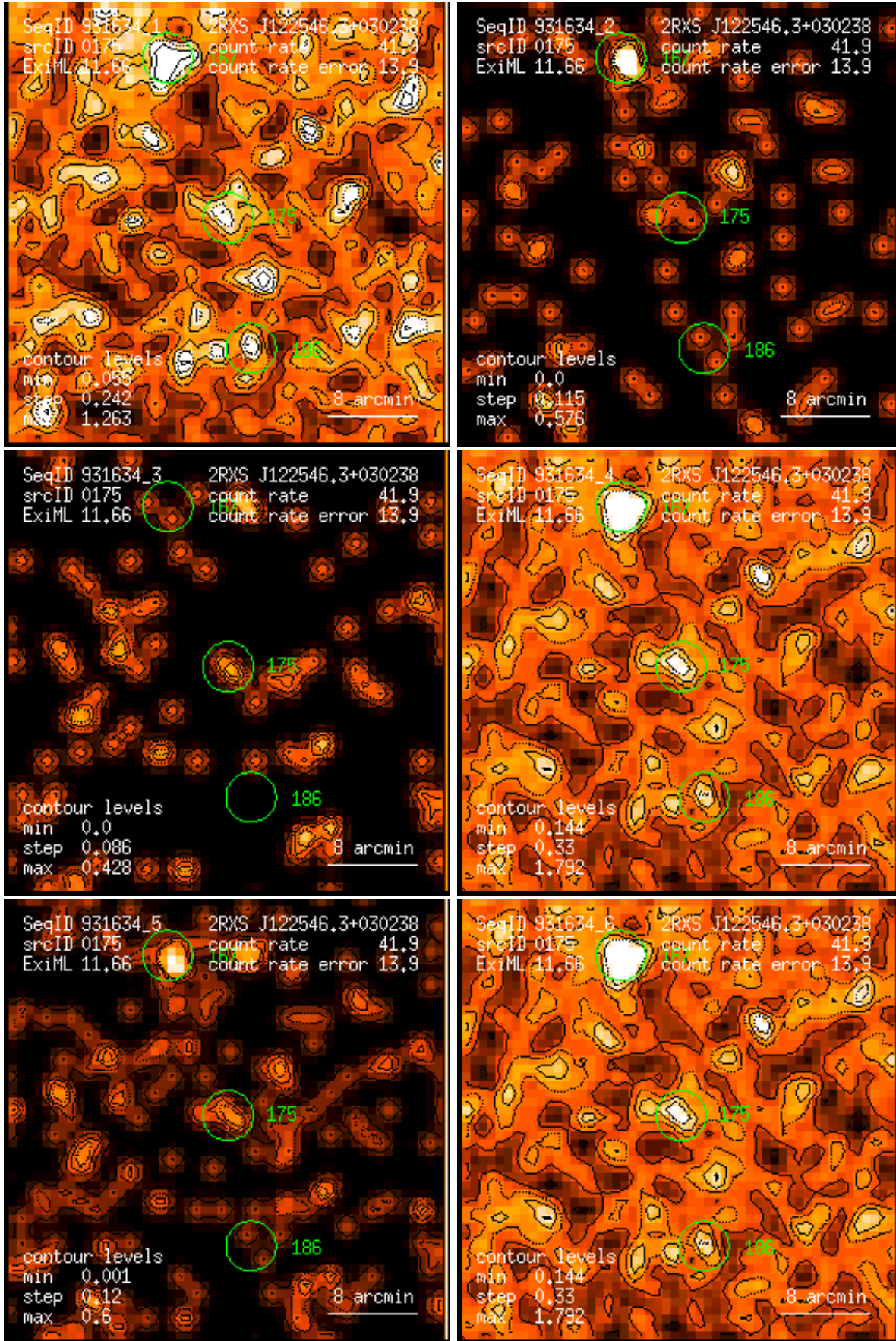
Figure 175: RASS 931634: detection 0175: band rate images, Gaussian filter: (1) PSPC channels 11 – 41, (2) 52 – 90, (3) 91 – 201, (4) 11 – 235, (5) 52 – 201, (6) 11 – 201. Broad band rates in counts/ks. Band rate contour levels in counts/ks/arcmin 2 .
