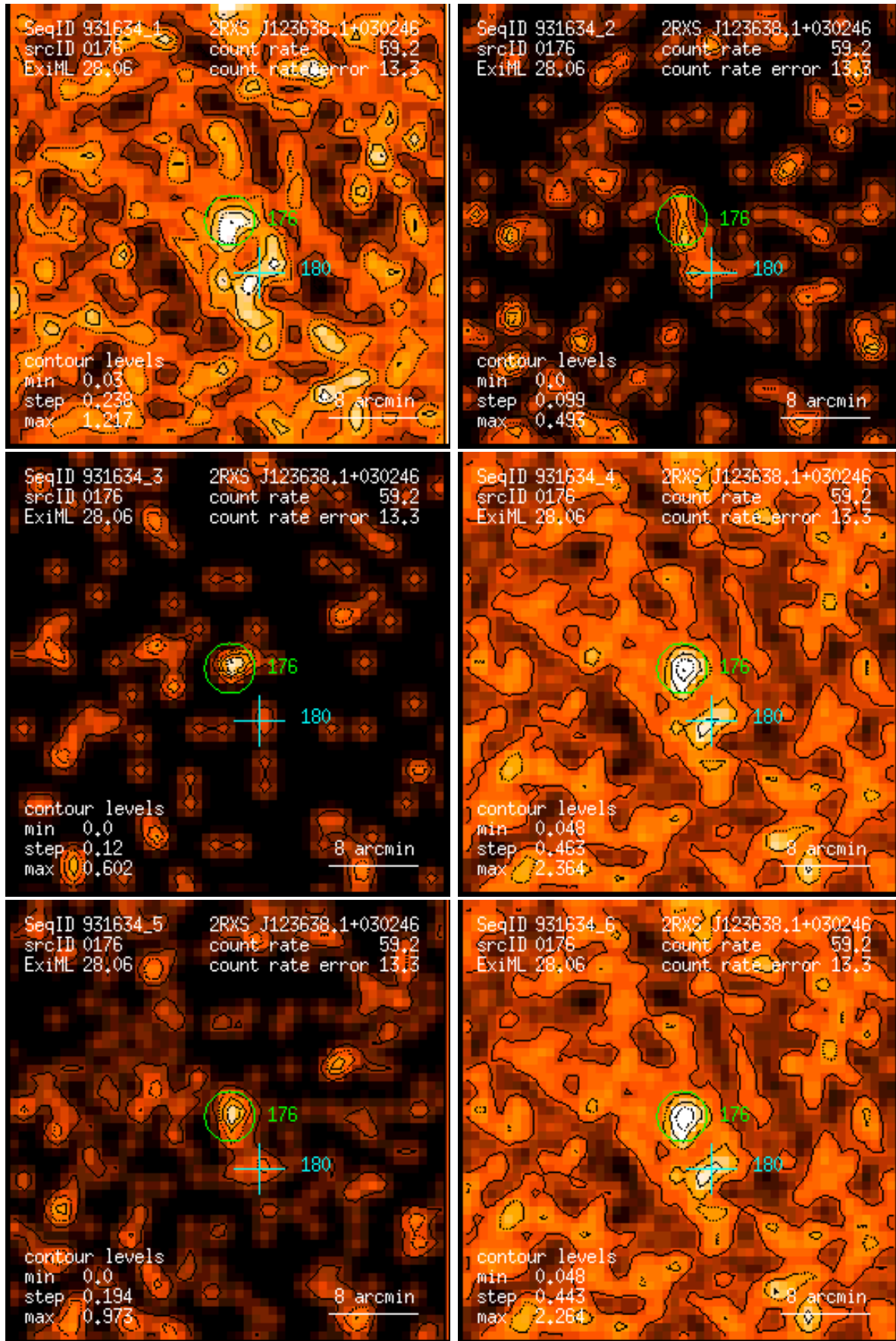
Figure 176: RASS 931634: detection 0176: band rate images, Gaussian filter: (1) PSPC channels 11 – 41, (2) 52 – 90, (3) 91 – 201, (4) 11 – 235, (5) 52 – 201, (6) 11 – 201. Broad band rates in counts/ks. Band rate contour levels in counts/ks/arcmin 2 .
