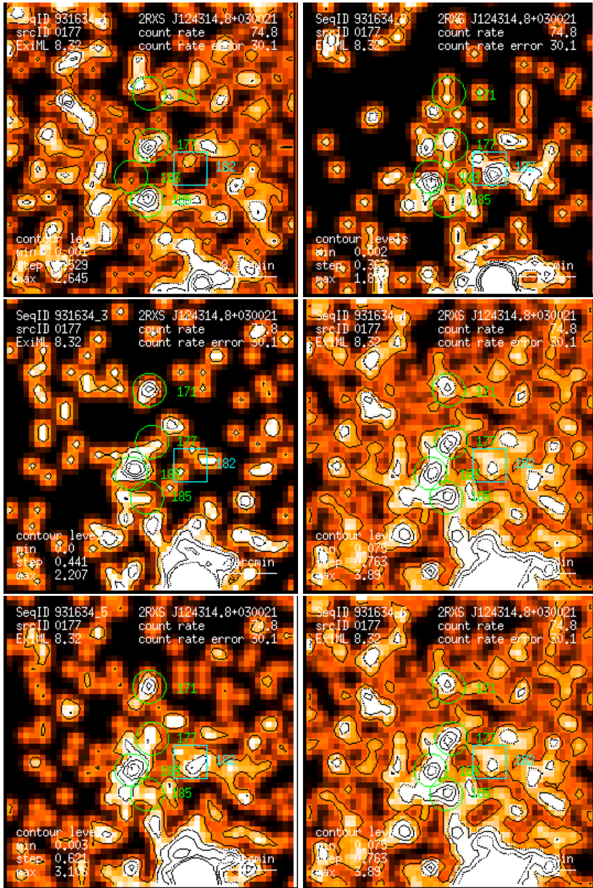
Figure 177: RASS 931634: detection 0177: band rate images, Gaussian filter: (1) PSPC channels 11 – 41, (2) 52 – 90, (3) 91 – 201, (4) 11 – 235, (5) 52 – 201, (6) 11 – 201. Broad band rates in counts/ks. Band rate contour levels in counts/ks/arcmin 2 .
