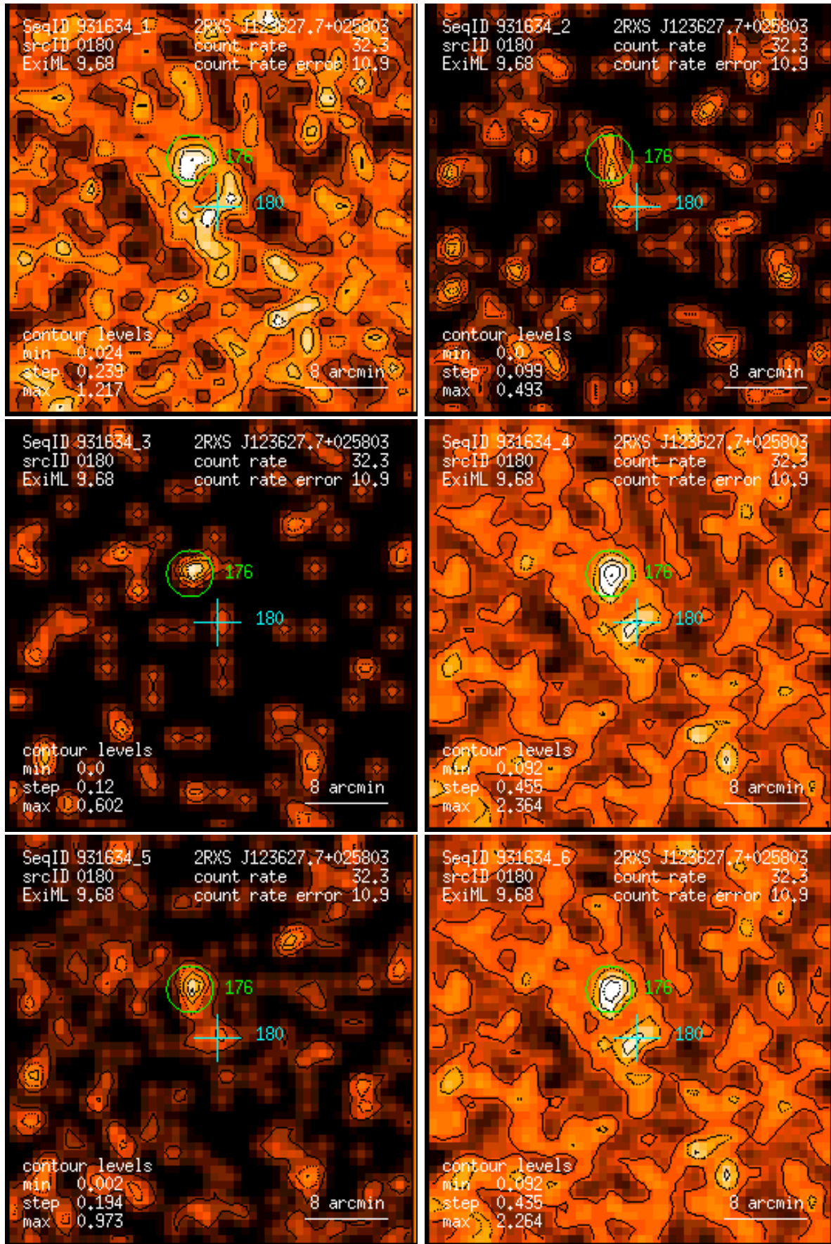
Figure 180: RASS 931634: detection 0180: band rate images, Gaussian filter: (1) PSPC channels 11 – 41, (2) 52 – 90, (3) 91 – 201, (4) 11 – 235, (5) 52 – 201, (6) 11 – 201. Broad band rates in counts/ks. Band rate contour levels in counts/ks/arcmin 2 .
