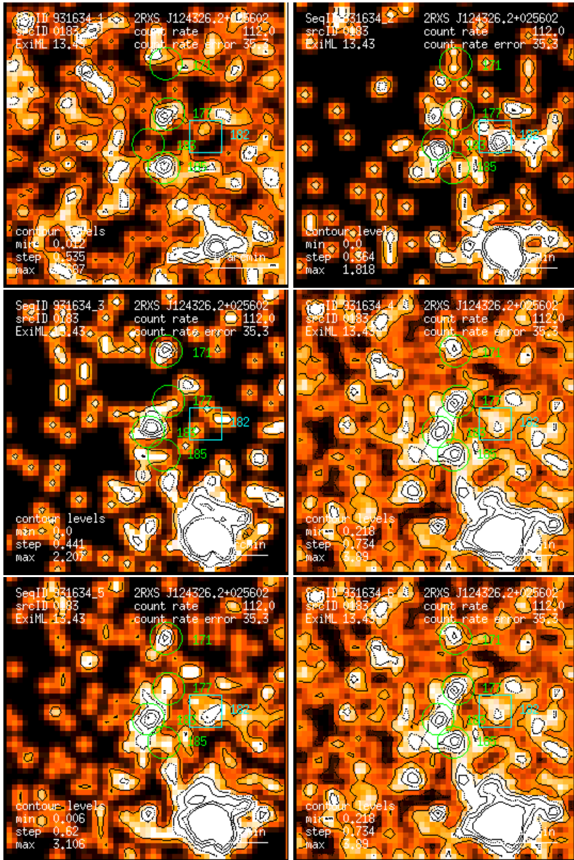
Figure 183: RASS 931634: detection 0183: band rate images, Gaussian filter: (1) PSPC channels 11 – 41, (2) 52 – 90, (3) 91 – 201, (4) 11 – 235, (5) 52 – 201, (6) 11 – 201. Broad band rates in counts/ks. Band rate contour levels in counts/ks/arcmin 2 .
