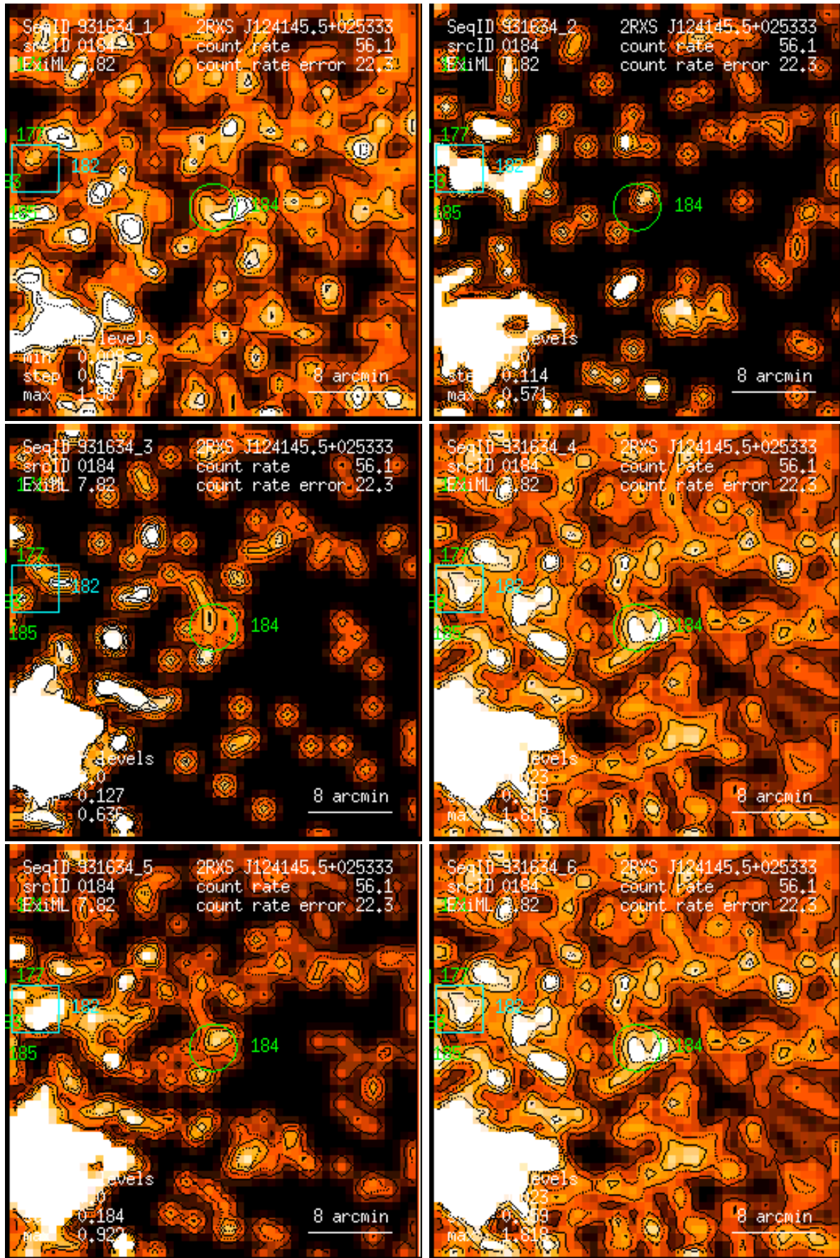
Figure 184: RASS 931634: detection 0184: band rate images, Gaussian filter: (1) PSPC channels 11 – 41, (2) 52 – 90, (3) 91 – 201, (4) 11 – 235, (5) 52 – 201, (6) 11 – 201. Broad band rates in counts/ks. Band rate contour levels in counts/ks/arcmin 2 .
