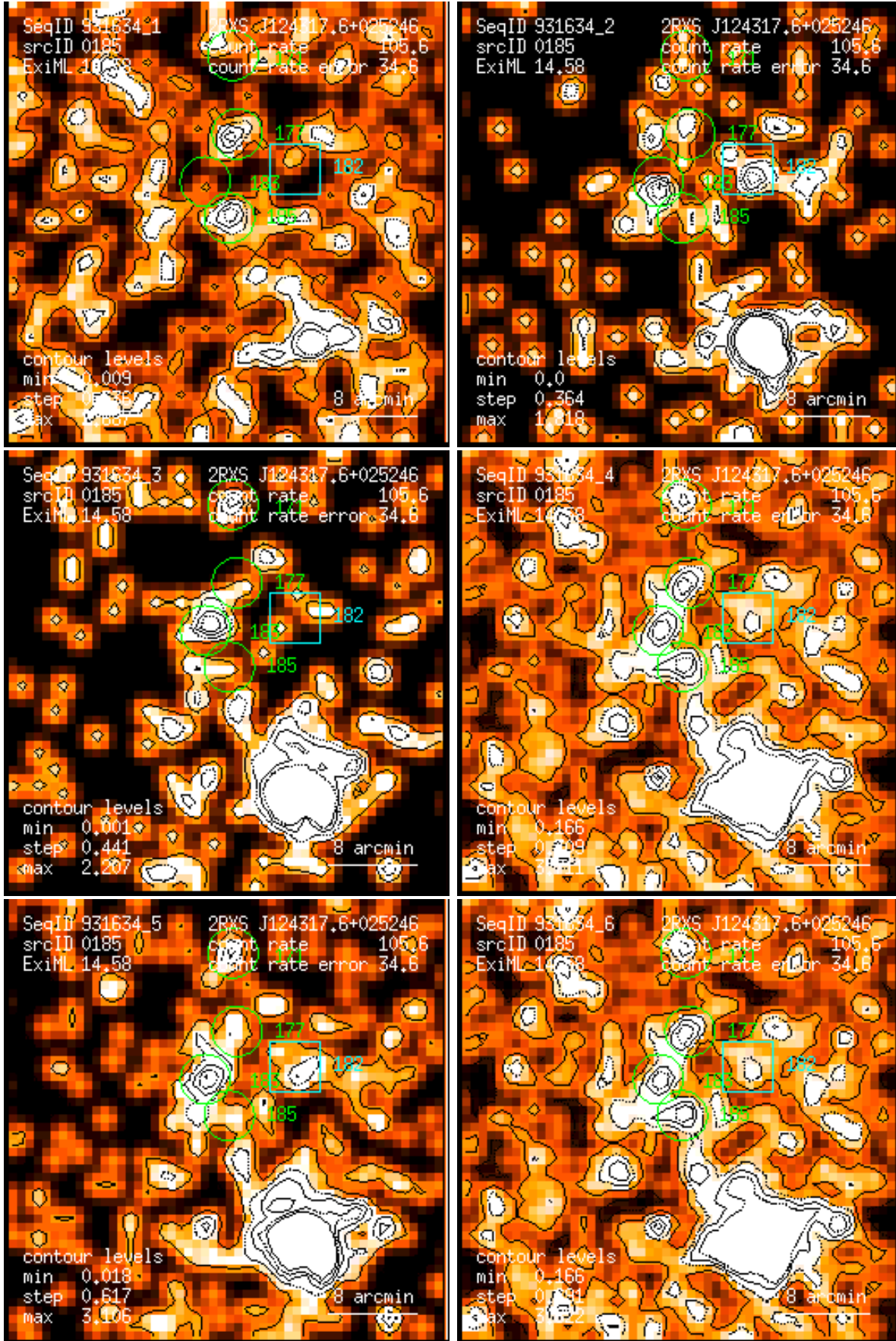
Figure 185: RASS 931634: detection 0185: band rate images, Gaussian filter: (1) PSPC channels 11 – 41, (2) 52 – 90, (3) 91 – 201, (4) 11 – 235, (5) 52 – 201, (6) 11 – 201. Broad band rates in counts/ks. Band rate contour levels in counts/ks/arcmin 2 .
