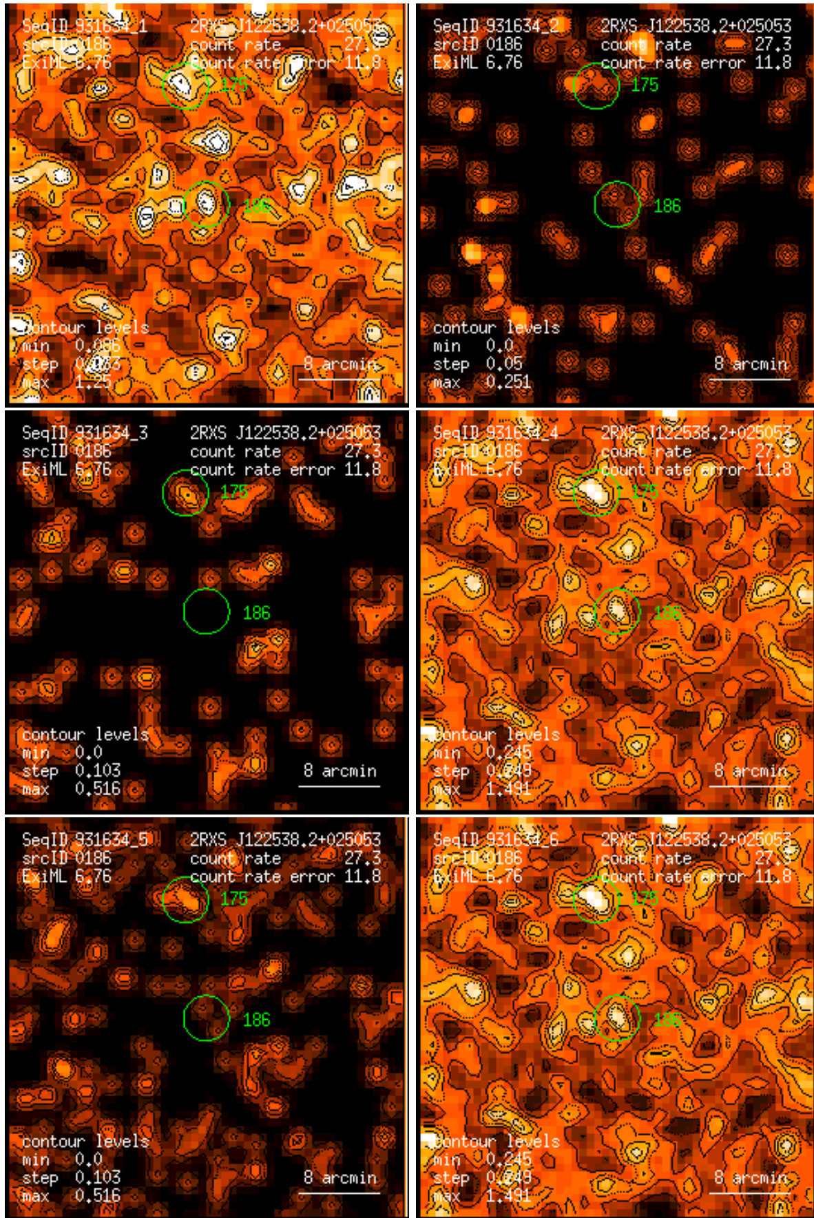
Figure 186: RASS 931634: detection 0186: band rate images, Gaussian filter: (1) PSPC channels 11 – 41, (2) 52 – 90, (3) 91 – 201, (4) 11 – 235, (5) 52 – 201, (6) 11 – 201. Broad band rates in counts/ks. Band rate contour levels in counts/ks/arcmin 2 .
