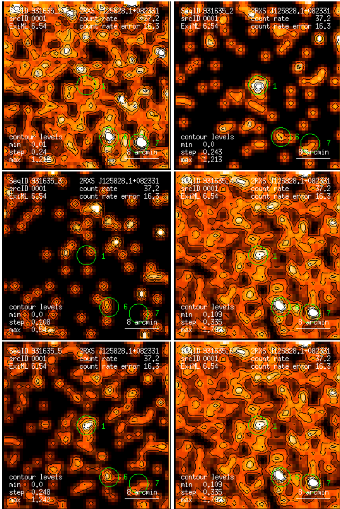
Figure 1: RASS 931635: detection 0001: band rate images, Gaussian filter: (1) PSPC channels 11 – 41, (2) 52 – 90, (3) 91 – 201, (4) 11 – 235, (5) 52 – 201, (6) 11 – 201. Broad band rates in counts/ks. Band rate contour levels in counts/ks/arcmin 2 .
