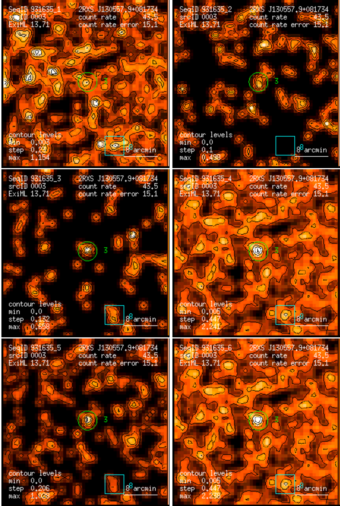
Figure 3: RASS 931635: detection 0003: band rate images, Gaussian filter: (1) PSPC channels 11 – 41, (2) 52 – 90, (3) 91 – 201, (4) 11 – 235, (5) 52 – 201, (6) 11 – 201. Broad band rates in counts/ks. Band rate contour levels in counts/ks/arcmin 2 .
