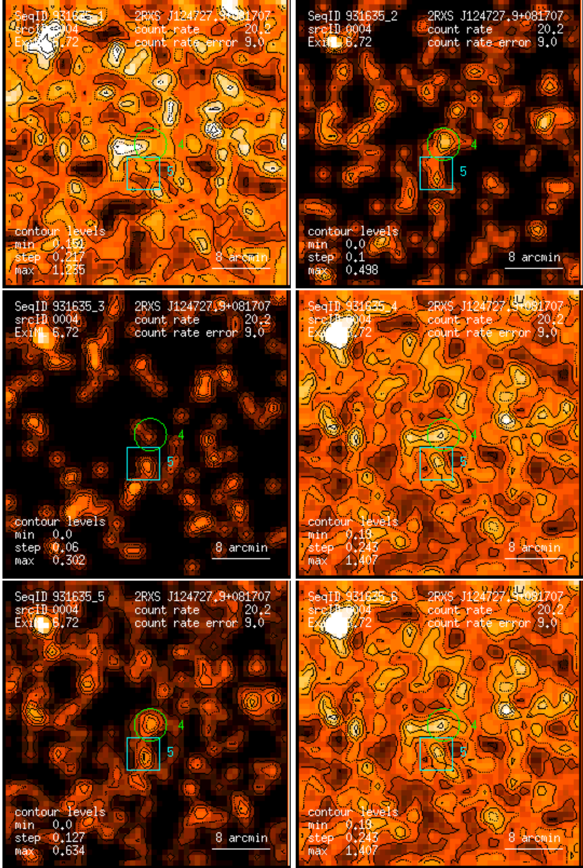
Figure 4: RASS 931635: detection 0004: band rate images, Gaussian filter: (1) PSPC channels 11 – 41, (2) 52 – 90, (3) 91 – 201, (4) 11 – 235, (5) 52 – 201, (6) 11 – 201. Broad band rates in counts/ks. Band rate contour levels in counts/ks/arcmin 2 .
