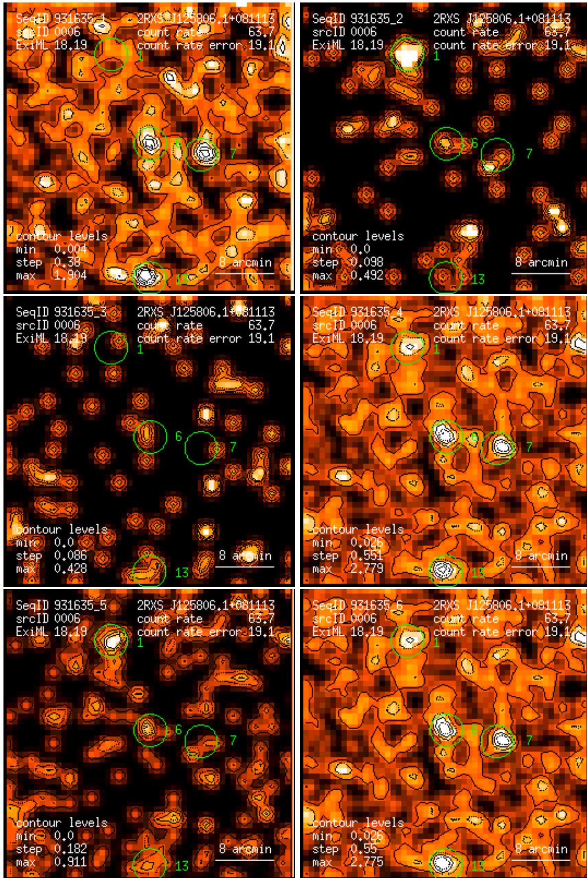
Figure 6: RASS 931635: detection 0006: band rate images, Gaussian filter: (1) PSPC channels 11 – 41, (2) 52 – 90, (3) 91 – 201, (4) 11 – 235, (5) 52 – 201, (6) 11 – 201. Broad band rates in counts/ks. Band rate contour levels in counts/ks/arcmin 2 .
