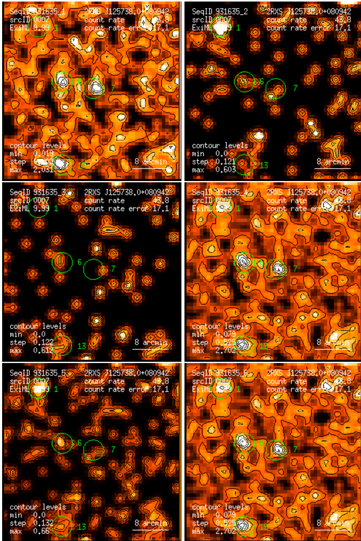
Figure 7: RASS 931635: detection 0007: band rate images, Gaussian filter: (1) PSPC channels 11 – 41, (2) 52 – 90, (3) 91 – 201, (4) 11 – 235, (5) 52 – 201, (6) 11 – 201. Broad band rates in counts/ks. Band rate contour levels in counts/ks/arcmin 2 .
