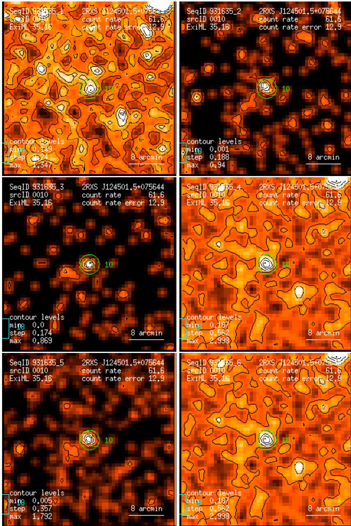
Figure 10: RASS 931635: detection 0010: band rate images, Gaussian filter: (1) PSPC channels 11 – 41, (2) 52 – 90, (3) 91 – 201, (4) 11 – 235, (5) 52 – 201, (6) 11 – 201. Broad band rates in counts/ks. Band rate contour levels in counts/ks/arcmin 2 .
