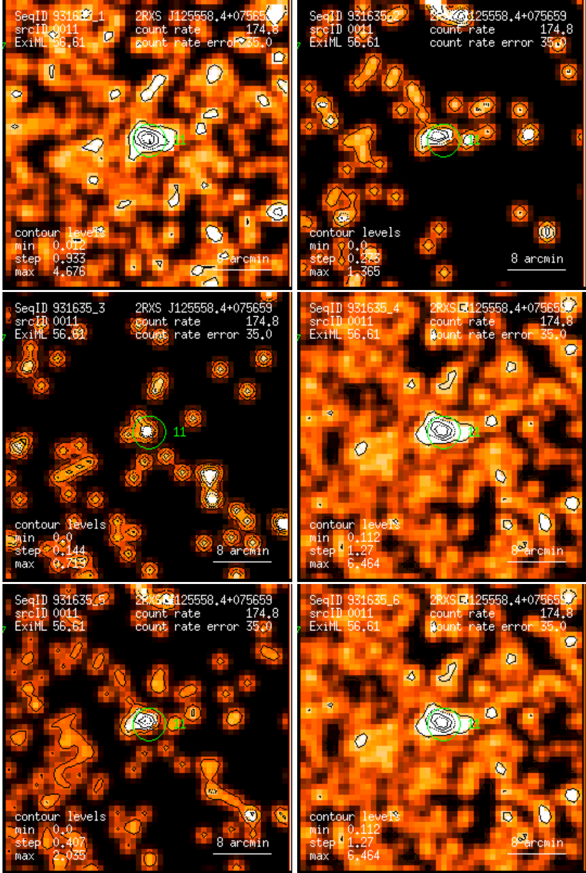
Figure 11: RASS 931635: detection 0011: band rate images, Gaussian filter: (1) PSPC channels 11 – 41, (2) 52 – 90, (3) 91 – 201, (4) 11 – 235, (5) 52 – 201, (6) 11 – 201. Broad band rates in counts/ks. Band rate contour levels in counts/ks/arcmin 2 .
