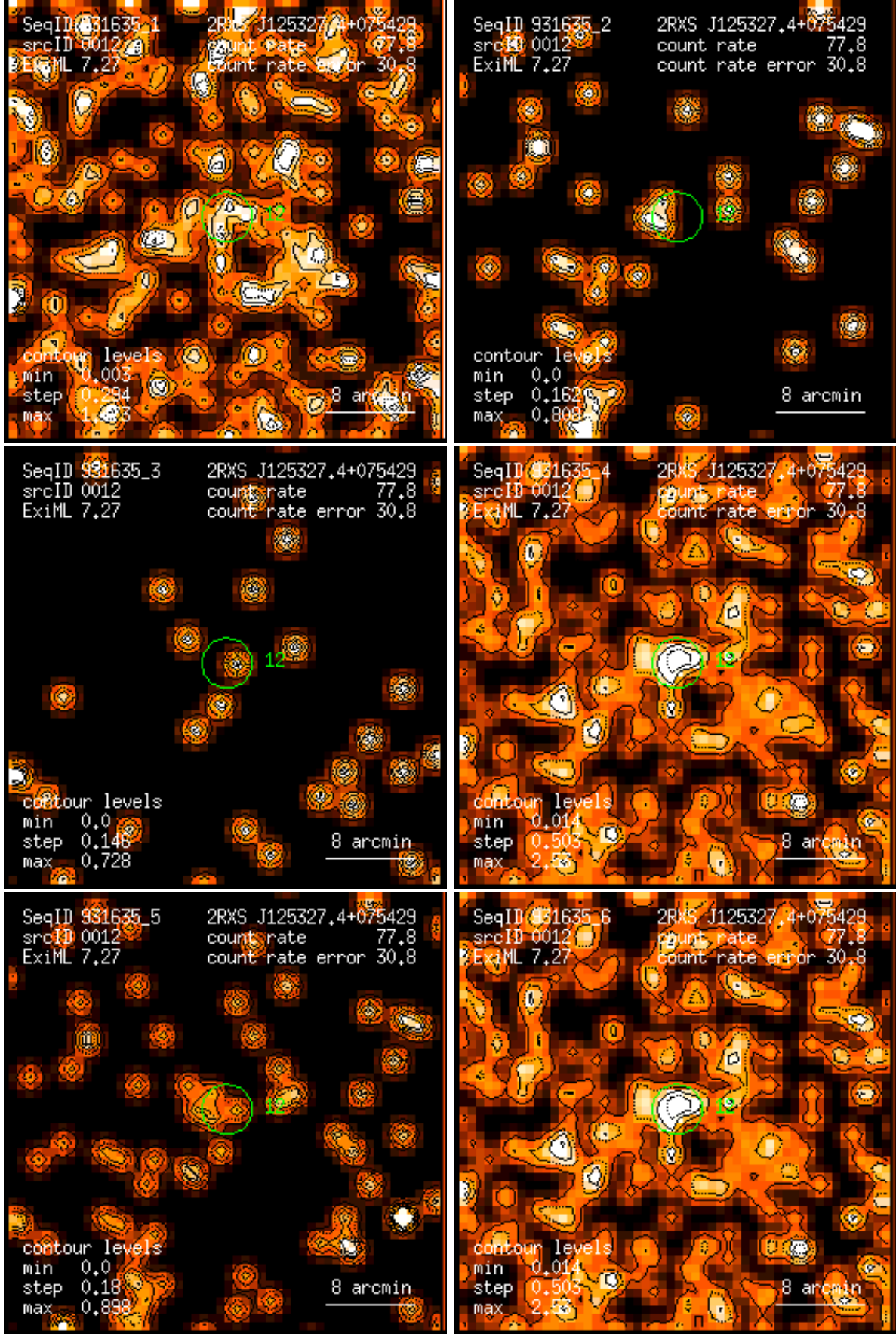
Figure 12: RASS 931635: detection 0012: band rate images, Gaussian filter: (1) PSPC channels 11 – 41, (2) 52 – 90, (3) 91 – 201, (4) 11 – 235, (5) 52 – 201, (6) 11 – 201. Broad band rates in counts/ks. Band rate contour levels in counts/ks/arcmin 2 .
