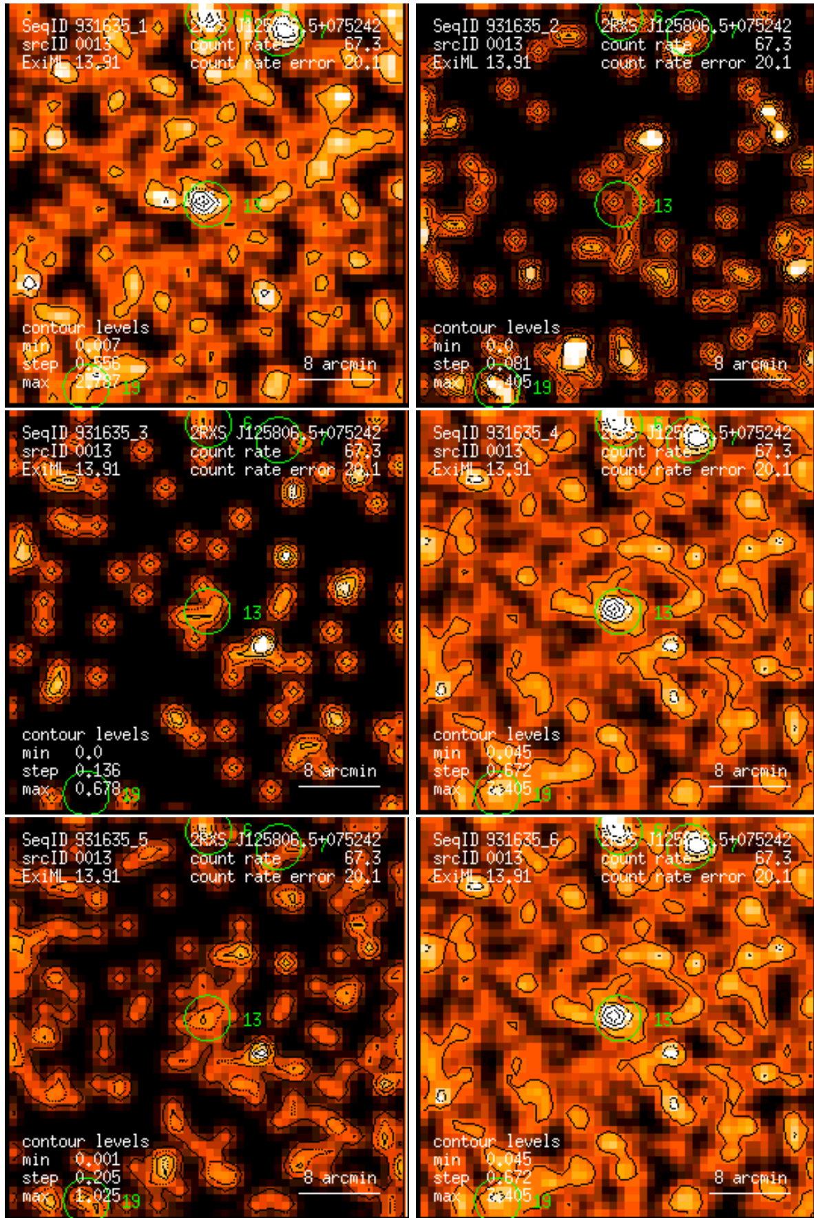
Figure 13: RASS 931635: detection 0013: band rate images, Gaussian filter: (1) PSPC channels 11 – 41, (2) 52 – 90, (3) 91 – 201, (4) 11 – 235, (5) 52 – 201, (6) 11 – 201. Broad band rates in counts/ks. Band rate contour levels in counts/ks/arcmin 2 .
