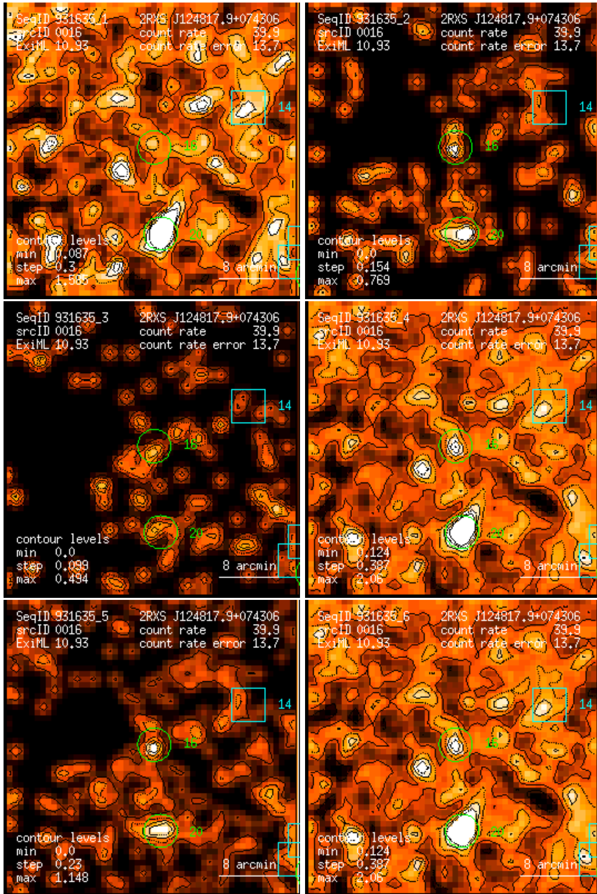
Figure 16: RASS 931635: detection 0016: band rate images, Gaussian filter: (1) PSPC channels 11 – 41, (2) 52 – 90, (3) 91 – 201, (4) 11 – 235, (5) 52 – 201, (6) 11 – 201. Broad band rates in counts/ks. Band rate contour levels in counts/ks/arcmin 2 .
