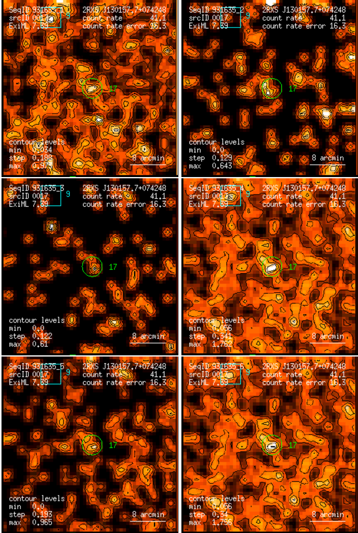
Figure 17: RASS 931635: detection 0017: band rate images, Gaussian filter: (1) PSPC channels 11 – 41, (2) 52 – 90, (3) 91 – 201, (4) 11 – 235, (5) 52 – 201, (6) 11 – 201. Broad band rates in counts/ks. Band rate contour levels in counts/ks/arcmin 2 .
