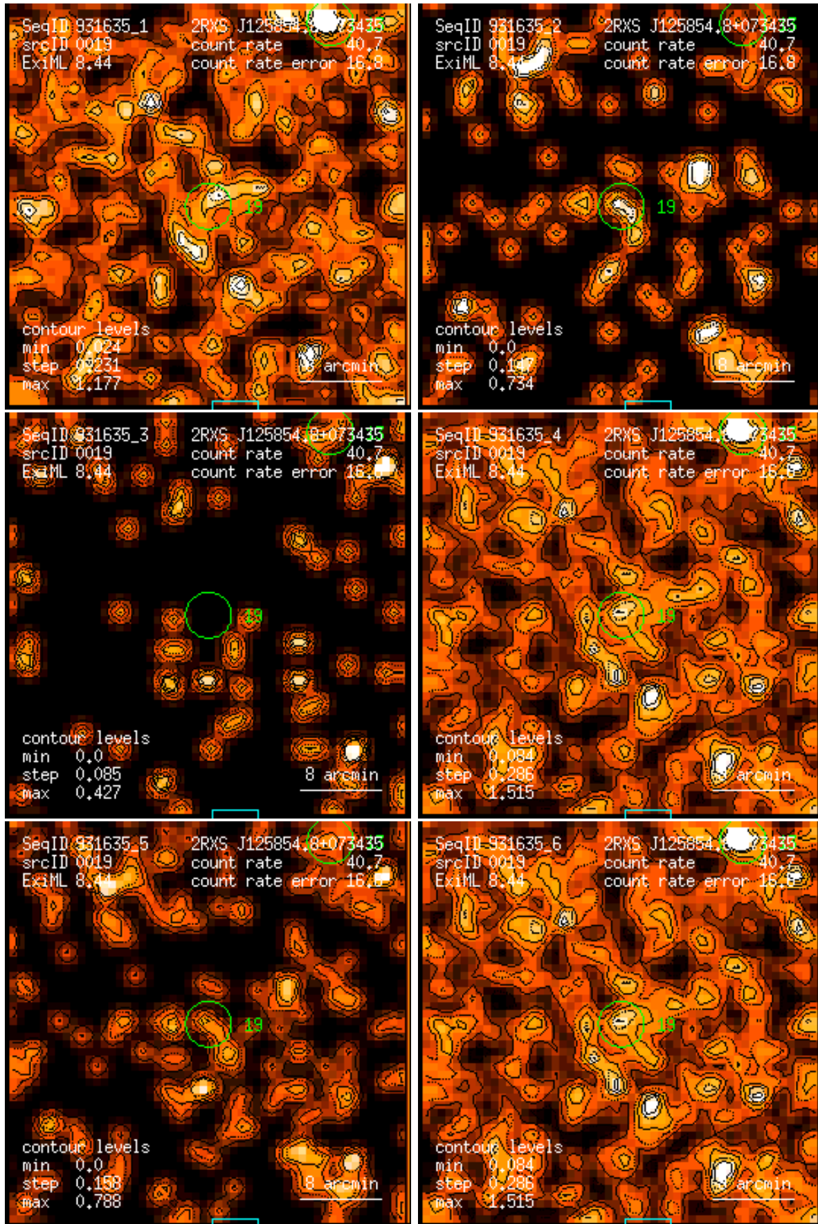
Figure 19: RASS 931635: detection 0019: band rate images, Gaussian filter: (1) PSPC channels 11 – 41, (2) 52 – 90, (3) 91 – 201, (4) 11 – 235, (5) 52 – 201, (6) 11 – 201. Broad band rates in counts/ks. Band rate contour levels in counts/ks/arcmin 2 .
