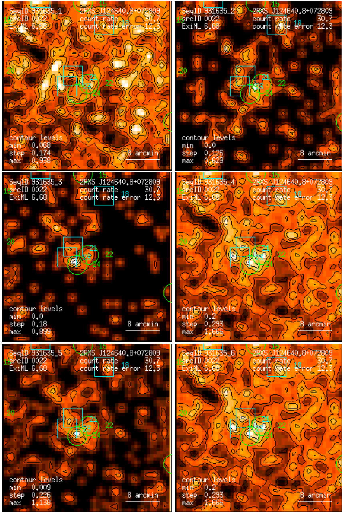
Figure 22: RASS 931635: detection 0022: band rate images, Gaussian filter: (1) PSPC channels 11 – 41, (2) 52 – 90, (3) 91 – 201, (4) 11 – 235, (5) 52 – 201, (6) 11 – 201. Broad band rates in counts/ks. Band rate contour levels in counts/ks/arcmin 2 .
