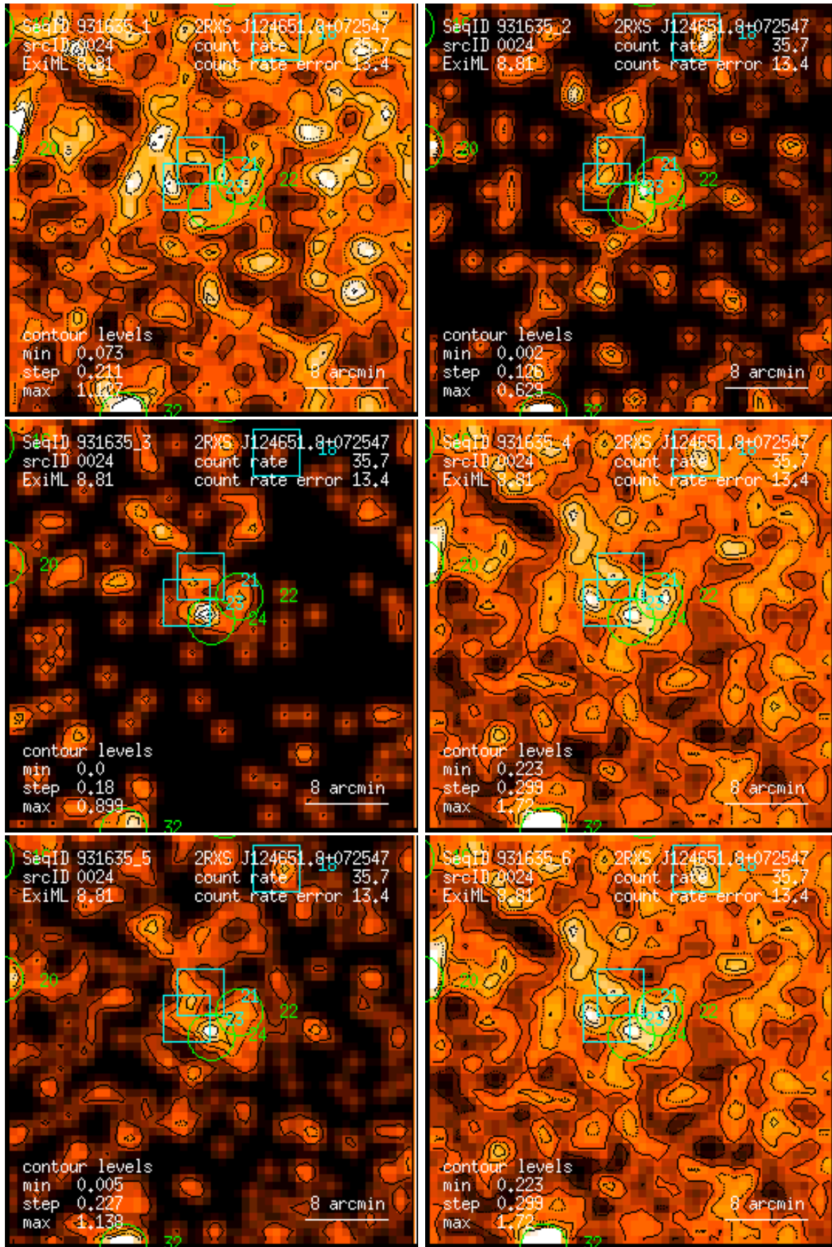
Figure 24: RASS 931635: detection 0024: band rate images, Gaussian filter: (1) PSPC channels 11 – 41, (2) 52 – 90, (3) 91 – 201, (4) 11 – 235, (5) 52 – 201, (6) 11 – 201. Broad band rates in counts/ks. Band rate contour levels in counts/ks/arcmin 2 .
