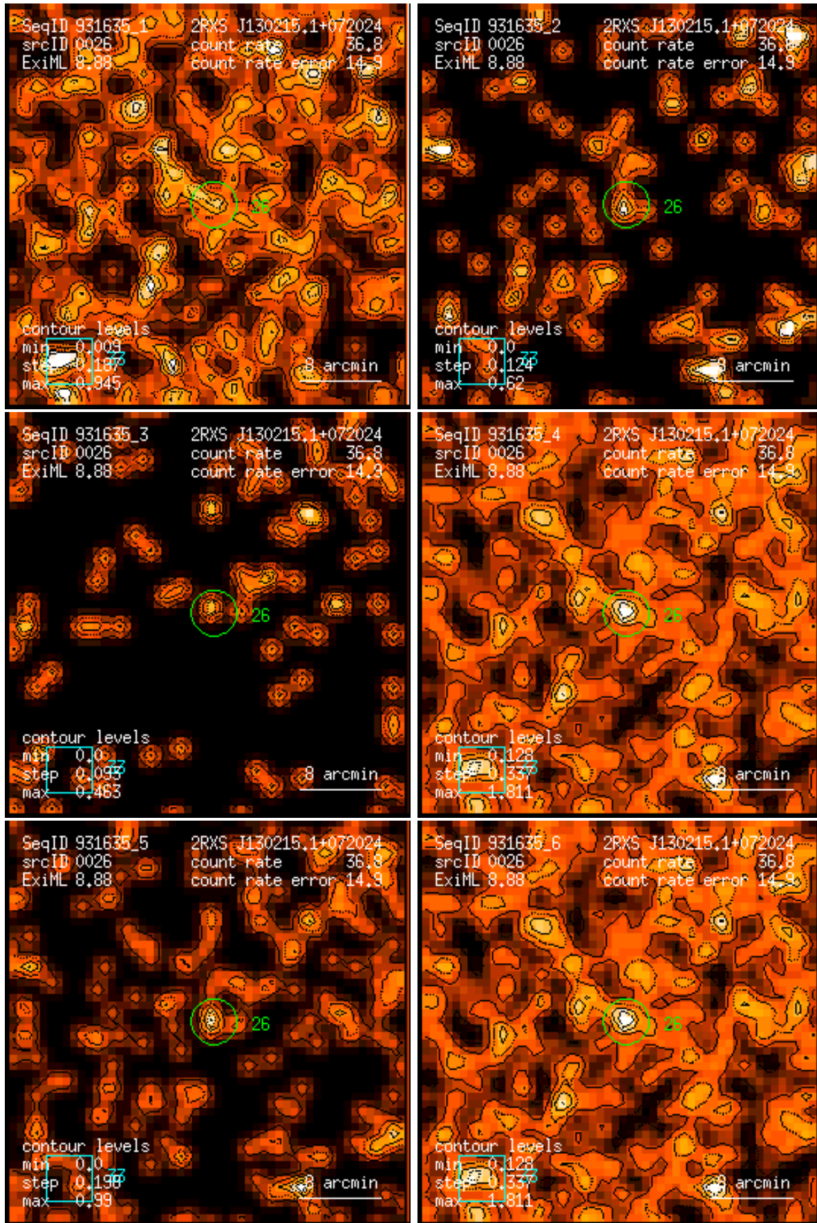
Figure 26: RASS 931635: detection 0026: band rate images, Gaussian filter: (1) PSPC channels 11 – 41, (2) 52 – 90, (3) 91 – 201, (4) 11 – 235, (5) 52 – 201, (6) 11 – 201. Broad band rates in counts/ks. Band rate contour levels in counts/ks/arcmin 2 .
