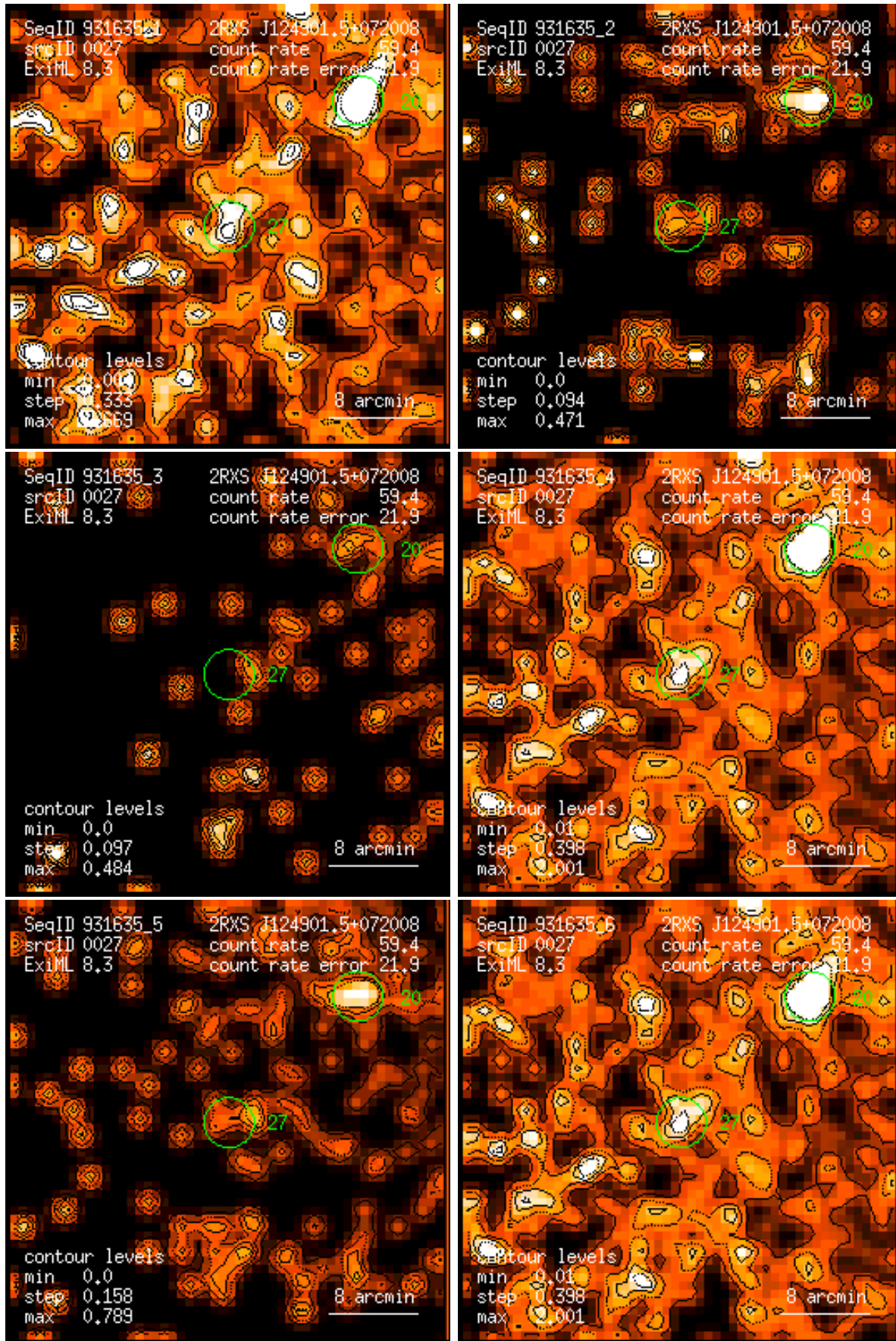
Figure 27: RASS 931635: detection 0027: band rate images, Gaussian filter: (1) PSPC channels 11 – 41, (2) 52 – 90, (3) 91 – 201, (4) 11 – 235, (5) 52 – 201, (6) 11 – 201. Broad band rates in counts/ks. Band rate contour levels in counts/ks/arcmin 2 .
