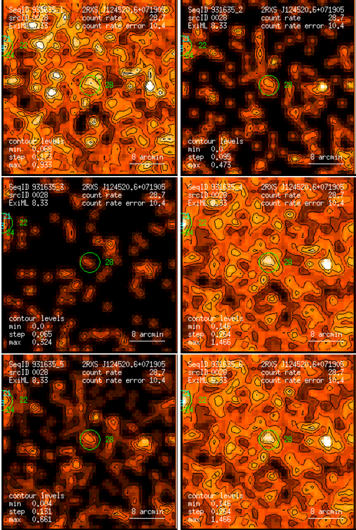
Figure 28: RASS 931635: detection 0028: band rate images, Gaussian filter: (1) PSPC channels 11 – 41, (2) 52 – 90, (3) 91 – 201, (4) 11 – 235, (5) 52 – 201, (6) 11 – 201. Broad band rates in counts/ks. Band rate contour levels in counts/ks/arcmin 2 .
