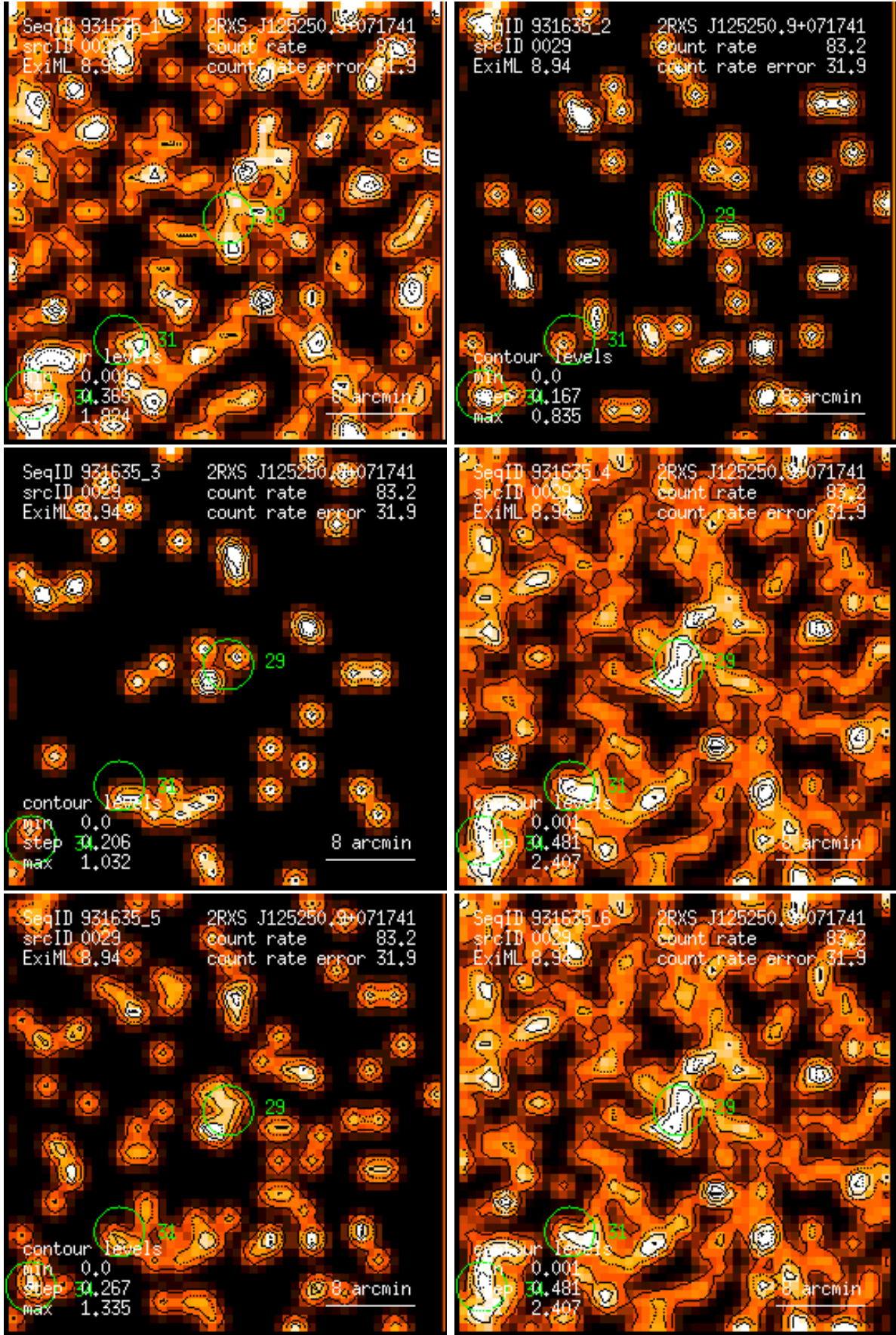
Figure 29: RASS 931635: detection 0029: band rate images, Gaussian filter: (1) PSPC channels 11 – 41, (2) 52 – 90, (3) 91 – 201, (4) 11 – 235, (5) 52 – 201, (6) 11 – 201. Broad band rates in counts/ks. Band rate contour levels in counts/ks/arcmin 2 .
