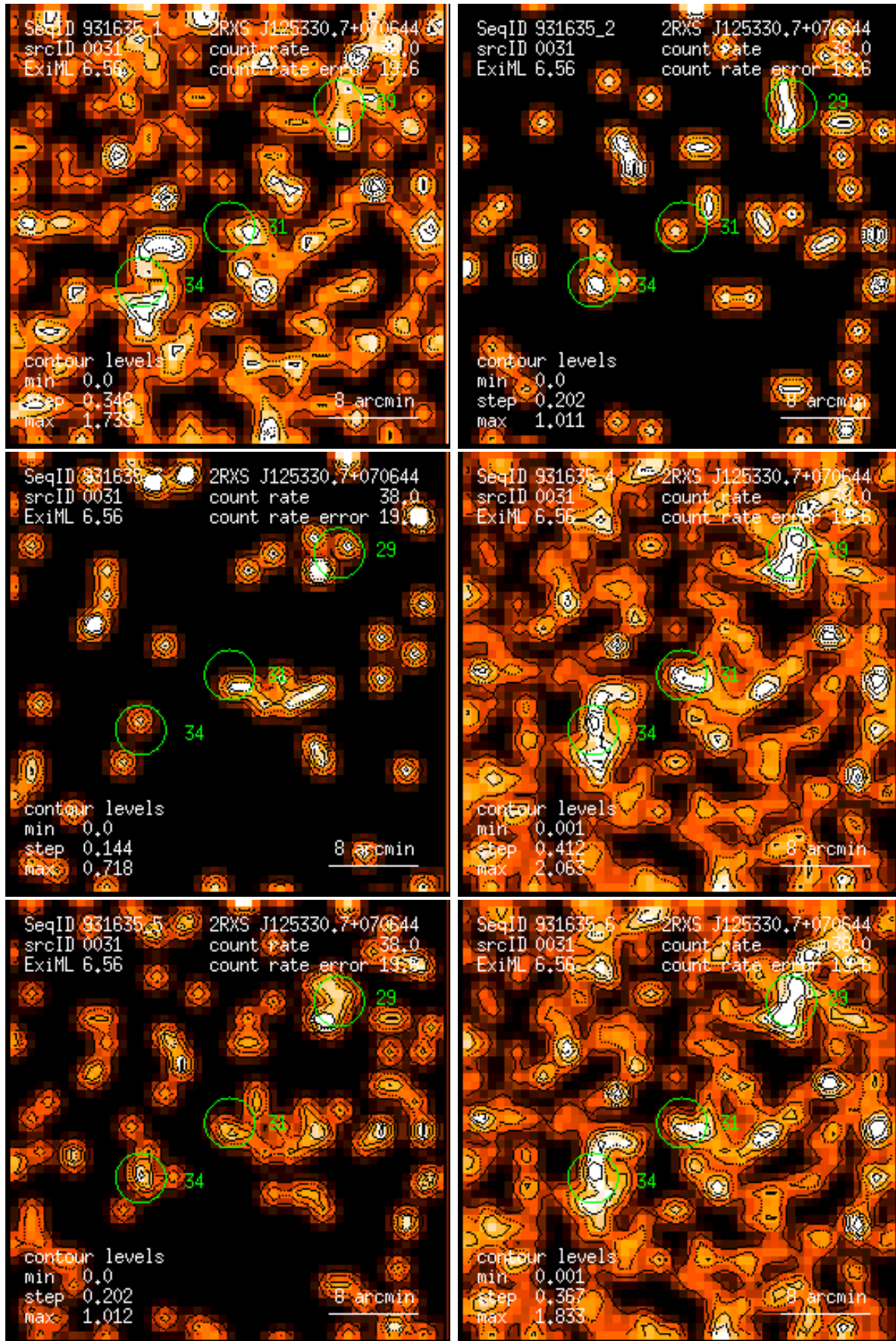
Figure 31: RASS 931635: detection 0031: band rate images, Gaussian filter: (1) PSPC channels 11 – 41, (2) 52 – 90, (3) 91 – 201, (4) 11 – 235, (5) 52 – 201, (6) 11 – 201. Broad band rates in counts/ks. Band rate contour levels in counts/ks/arcmin 2 .
