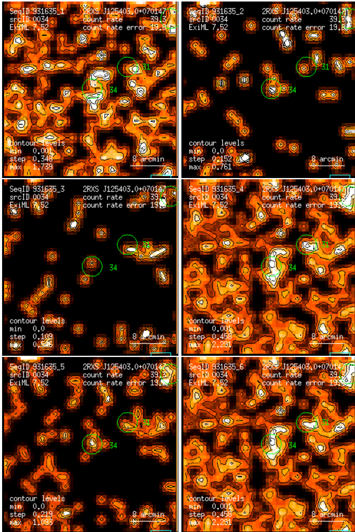
Figure 34: RASS 931635: detection 0034: band rate images, Gaussian filter: (1) PSPC channels 11 – 41, (2) 52 – 90, (3) 91 – 201, (4) 11 – 235, (5) 52 – 201, (6) 11 – 201. Broad band rates in counts/ks. Band rate contour levels in counts/ks/arcmin 2 .
