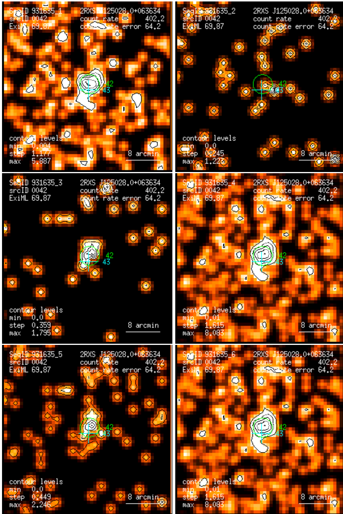
Figure 42: RASS 931635: detection 0042: band rate images, Gaussian filter: (1) PSPC channels 11 – 41, (2) 52 – 90, (3) 91 – 201, (4) 11 – 235, (5) 52 – 201, (6) 11 – 201. Broad band rates in counts/ks. Band rate contour levels in counts/ks/arcmin 2 .
