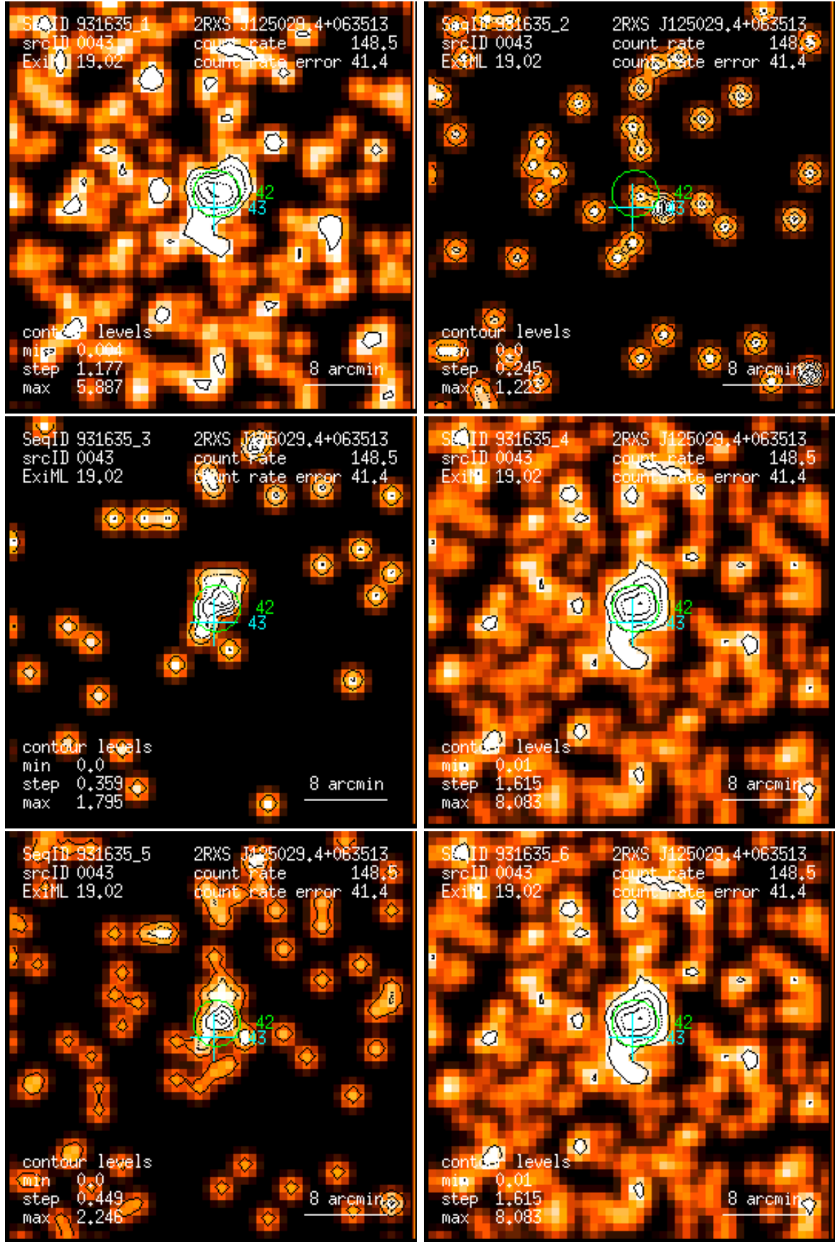
Figure 43: RASS 931635: detection 0043: band rate images, Gaussian filter: (1) PSPC channels 11 – 41, (2) 52 – 90, (3) 91 – 201, (4) 11 – 235, (5) 52 – 201, (6) 11 – 201. Broad band rates in counts/ks. Band rate contour levels in counts/ks/arcmin 2 .
