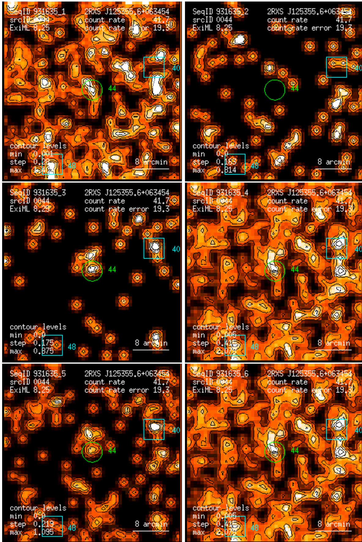
Figure 44: RASS 931635: detection 0044: band rate images, Gaussian filter: (1) PSPC channels 11 – 41, (2) 52 – 90, (3) 91 – 201, (4) 11 – 235, (5) 52 – 201, (6) 11 – 201. Broad band rates in counts/ks. Band rate contour levels in counts/ks/arcmin 2 .
