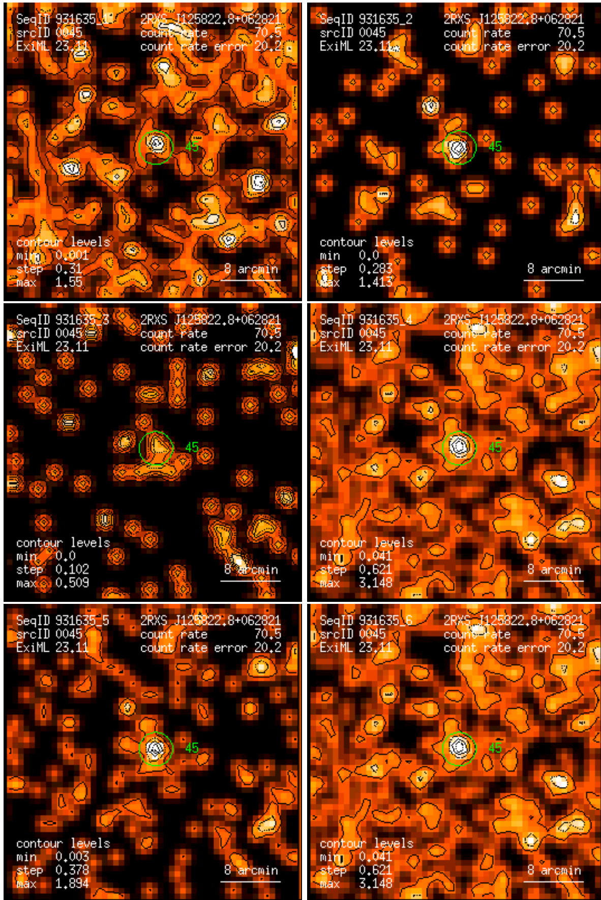
Figure 45: RASS 931635: detection 0045: band rate images, Gaussian filter: (1) PSPC channels 11 – 41, (2) 52 – 90, (3) 91 – 201, (4) 11 – 235, (5) 52 – 201, (6) 11 – 201. Broad band rates in counts/ks. Band rate contour levels in counts/ks/arcmin 2 .
