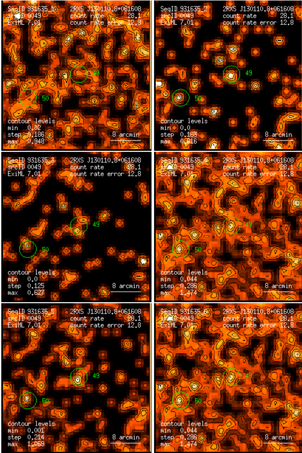
Figure 49: RASS 931635: detection 0049: band rate images, Gaussian filter: (1) PSPC channels 11 – 41, (2) 52 – 90, (3) 91 – 201, (4) 11 – 235, (5) 52 – 201, (6) 11 – 201. Broad band rates in counts/ks. Band rate contour levels in counts/ks/arcmin 2 .
