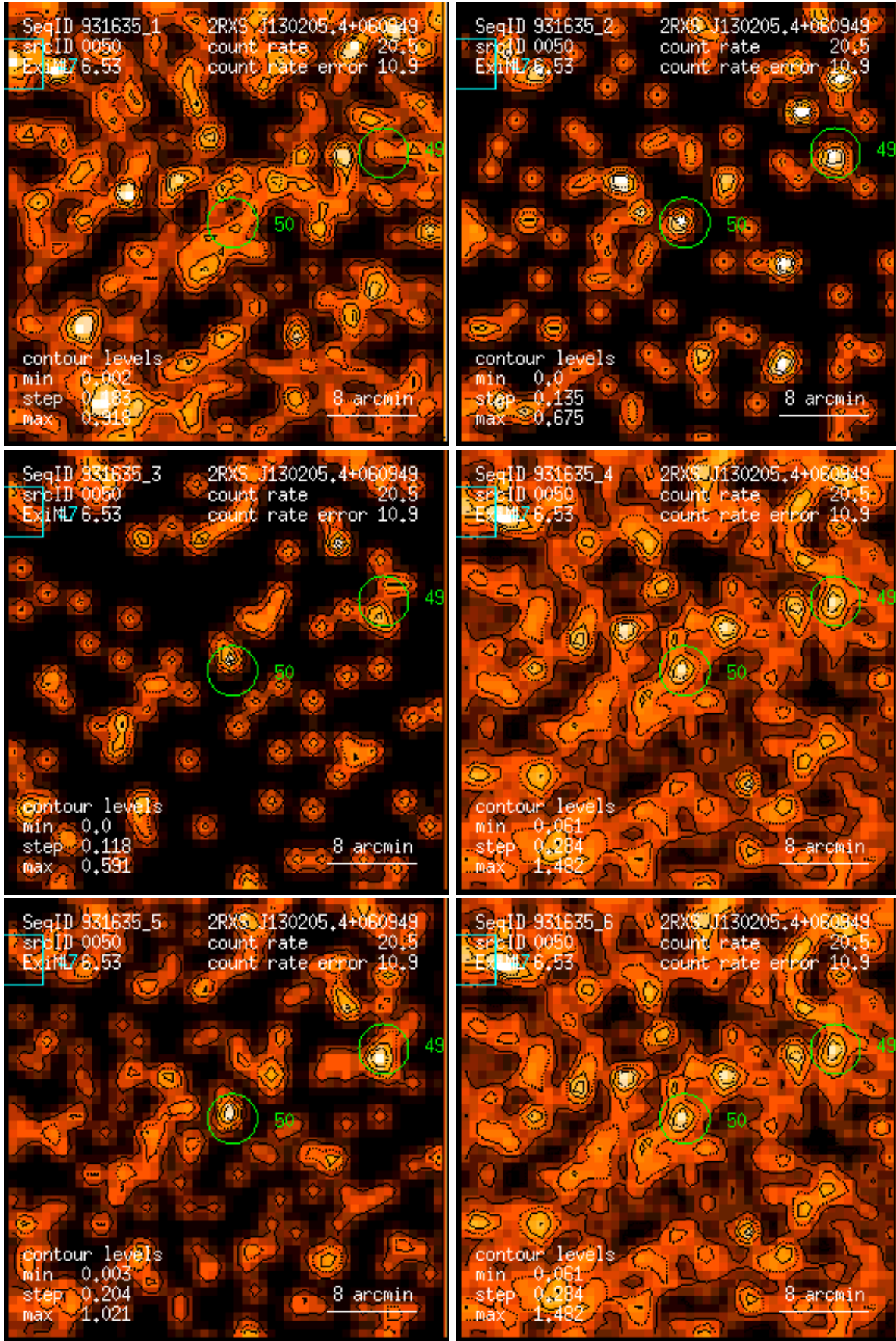
Figure 50: RASS 931635: detection 0050: band rate images, Gaussian filter: (1) PSPC channels 11 – 41, (2) 52 – 90, (3) 91 – 201, (4) 11 – 235, (5) 52 – 201, (6) 11 – 201. Broad band rates in counts/ks. Band rate contour levels in counts/ks/arcmin 2 .
