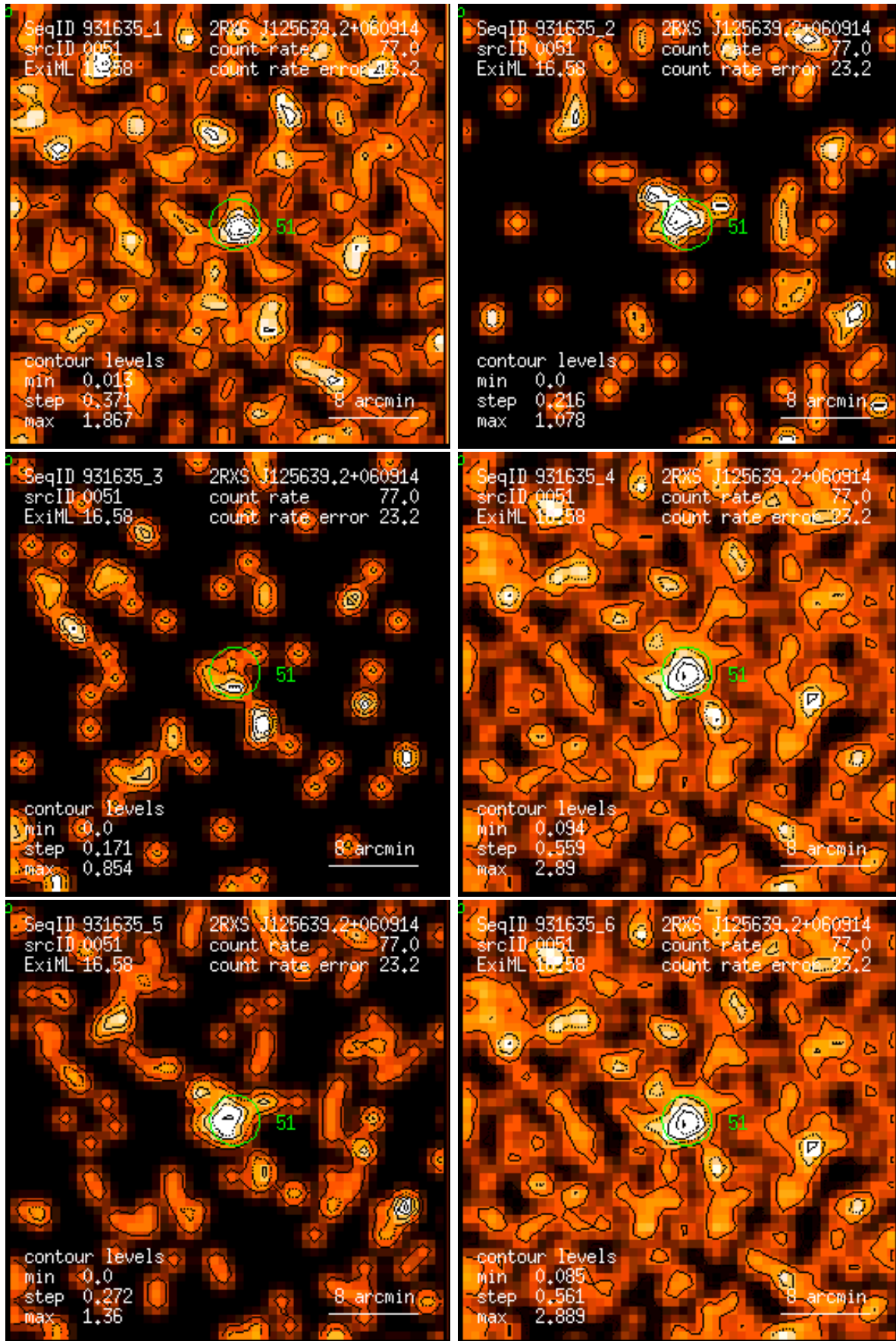
Figure 51: RASS 931635: detection 0051: band rate images, Gaussian filter: (1) PSPC channels 11 – 41, (2) 52 – 90, (3) 91 – 201, (4) 11 – 235, (5) 52 – 201, (6) 11 – 201. Broad band rates in counts/ks. Band rate contour levels in counts/ks/arcmin 2 .
