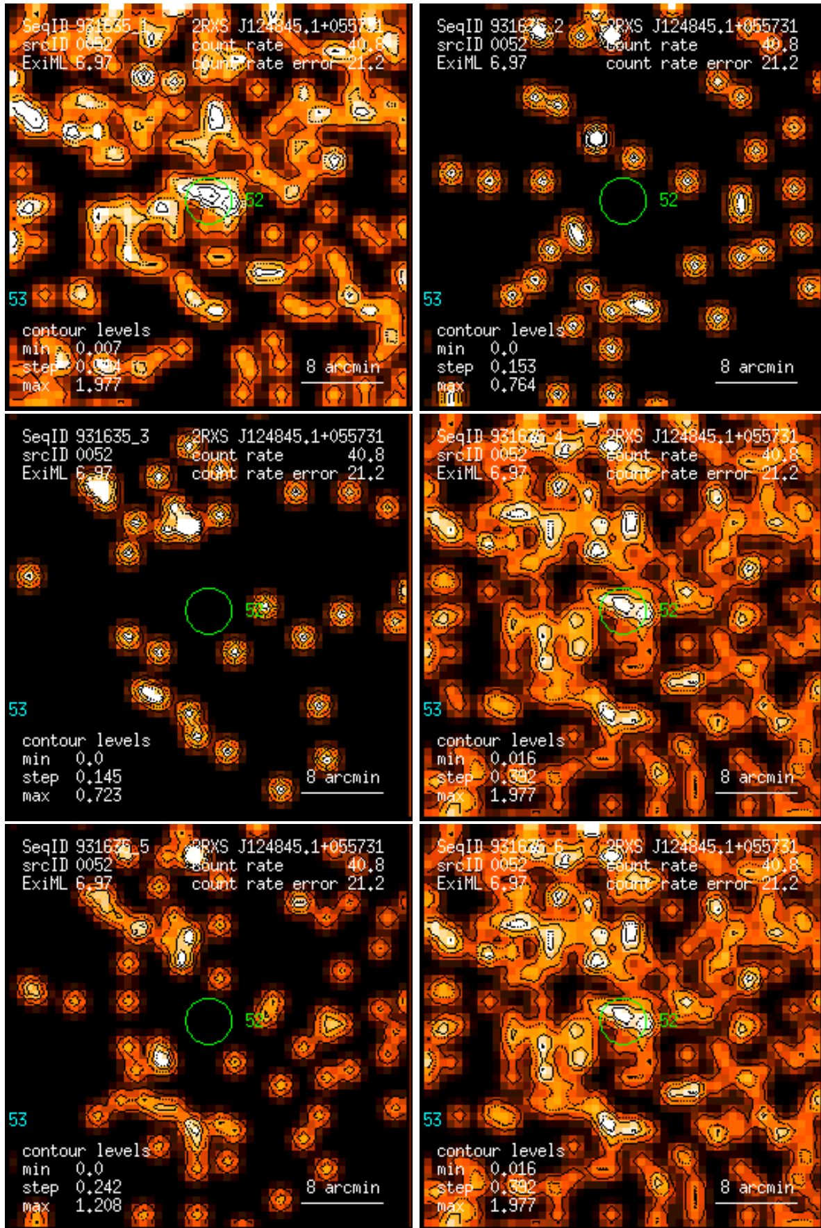
Figure 52: RASS 931635: detection 0052: band rate images, Gaussian filter: (1) PSPC channels 11 – 41, (2) 52 – 90, (3) 91 – 201, (4) 11 – 235, (5) 52 – 201, (6) 11 – 201. Broad band rates in counts/ks. Band rate contour levels in counts/ks/arcmin 2 .
