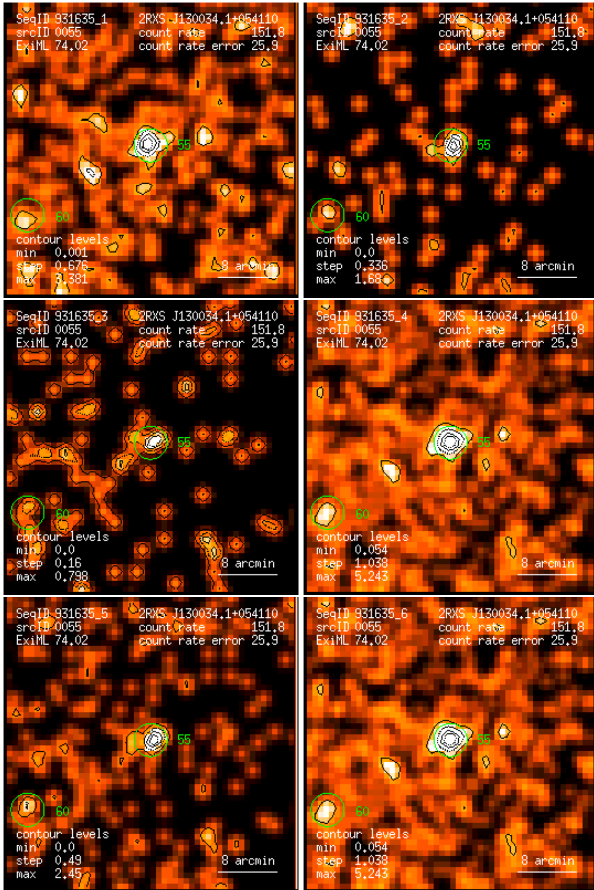
Figure 55: RASS 931635: detection 0055: band rate images, Gaussian filter: (1) PSPC channels 11 – 41, (2) 52 – 90, (3) 91 – 201, (4) 11 – 235, (5) 52 – 201, (6) 11 – 201. Broad band rates in counts/ks. Band rate contour levels in counts/ks/arcmin 2 .
