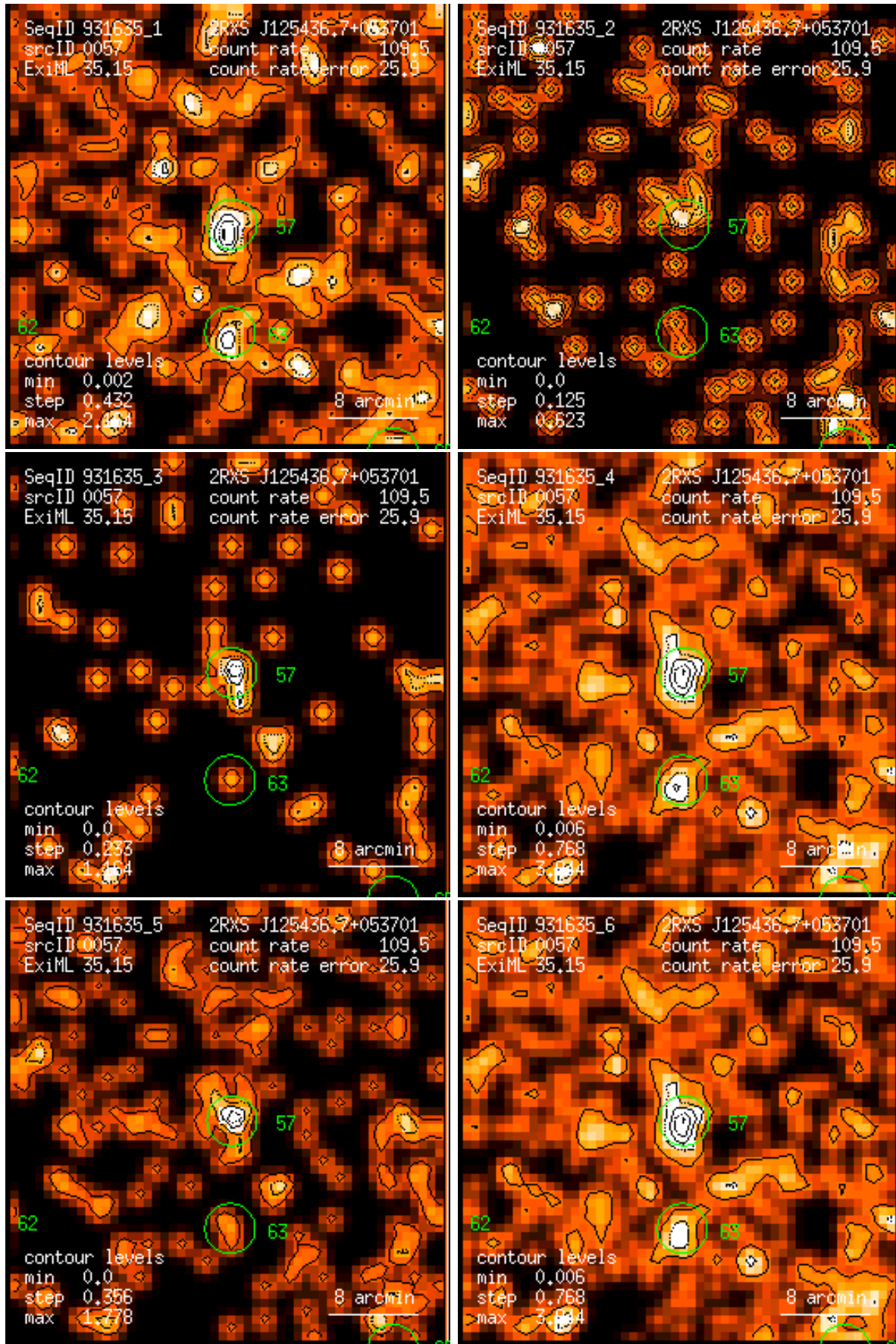
Figure 57: RASS 931635: detection 0057: band rate images, Gaussian filter: (1) PSPC channels 11 – 41, (2) 52 – 90, (3) 91 – 201, (4) 11 – 235, (5) 52 – 201, (6) 11 – 201. Broad band rates in counts/ks. Band rate contour levels in counts/ks/arcmin 2 .
