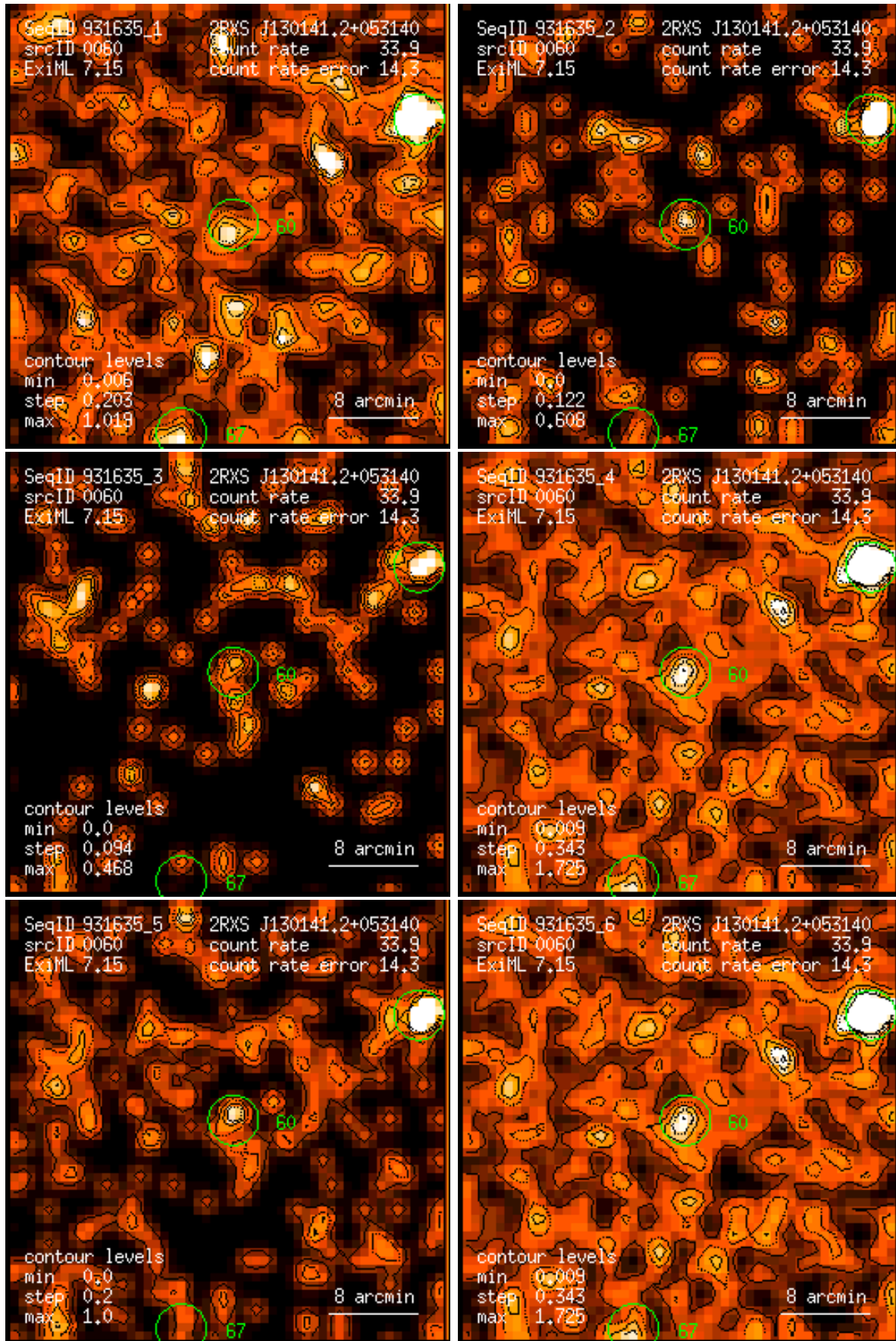
Figure 60: RASS 931635: detection 0060: band rate images, Gaussian filter: (1) PSPC channels 11 – 41, (2) 52 – 90, (3) 91 – 201, (4) 11 – 235, (5) 52 – 201, (6) 11 – 201. Broad band rates in counts/ks. Band rate contour levels in counts/ks/arcmin 2 .
