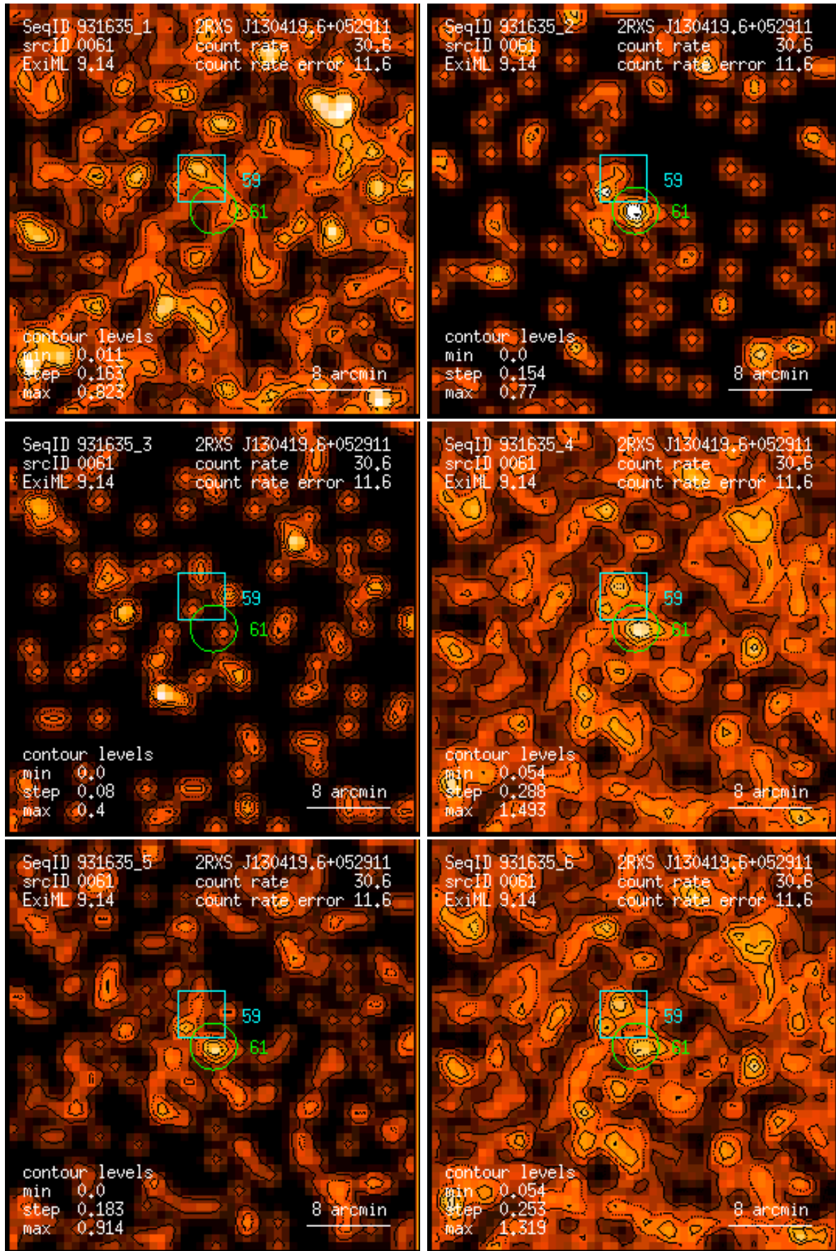
Figure 61: RASS 931635: detection 0061: band rate images, Gaussian filter: (1) PSPC channels 11 – 41, (2) 52 – 90, (3) 91 – 201, (4) 11 – 235, (5) 52 – 201, (6) 11 – 201. Broad band rates in counts/ks. Band rate contour levels in counts/ks/arcmin 2 .
