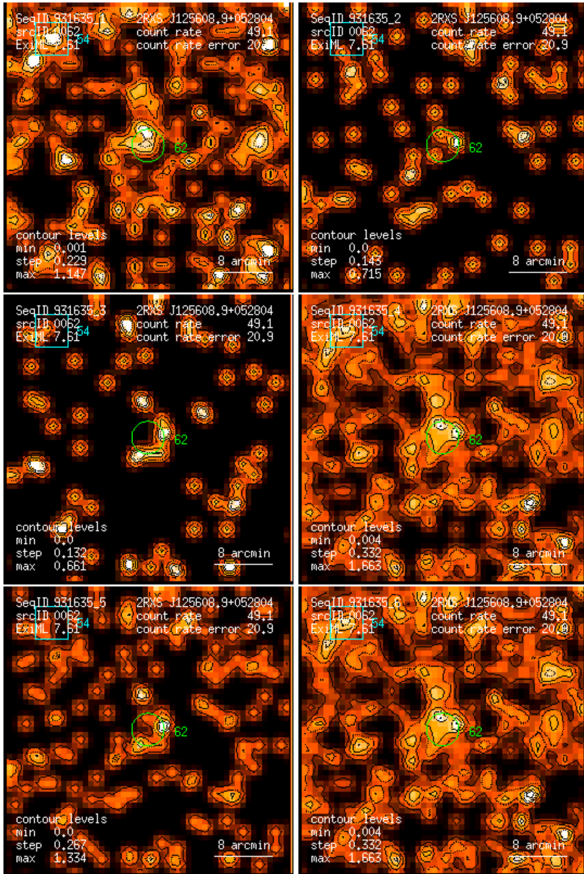
Figure 62: RASS 931635: detection 0062: band rate images, Gaussian filter: (1) PSPC channels 11 – 41, (2) 52 – 90, (3) 91 – 201, (4) 11 – 235, (5) 52 – 201, (6) 11 – 201. Broad band rates in counts/ks. Band rate contour levels in counts/ks/arcmin 2 .
