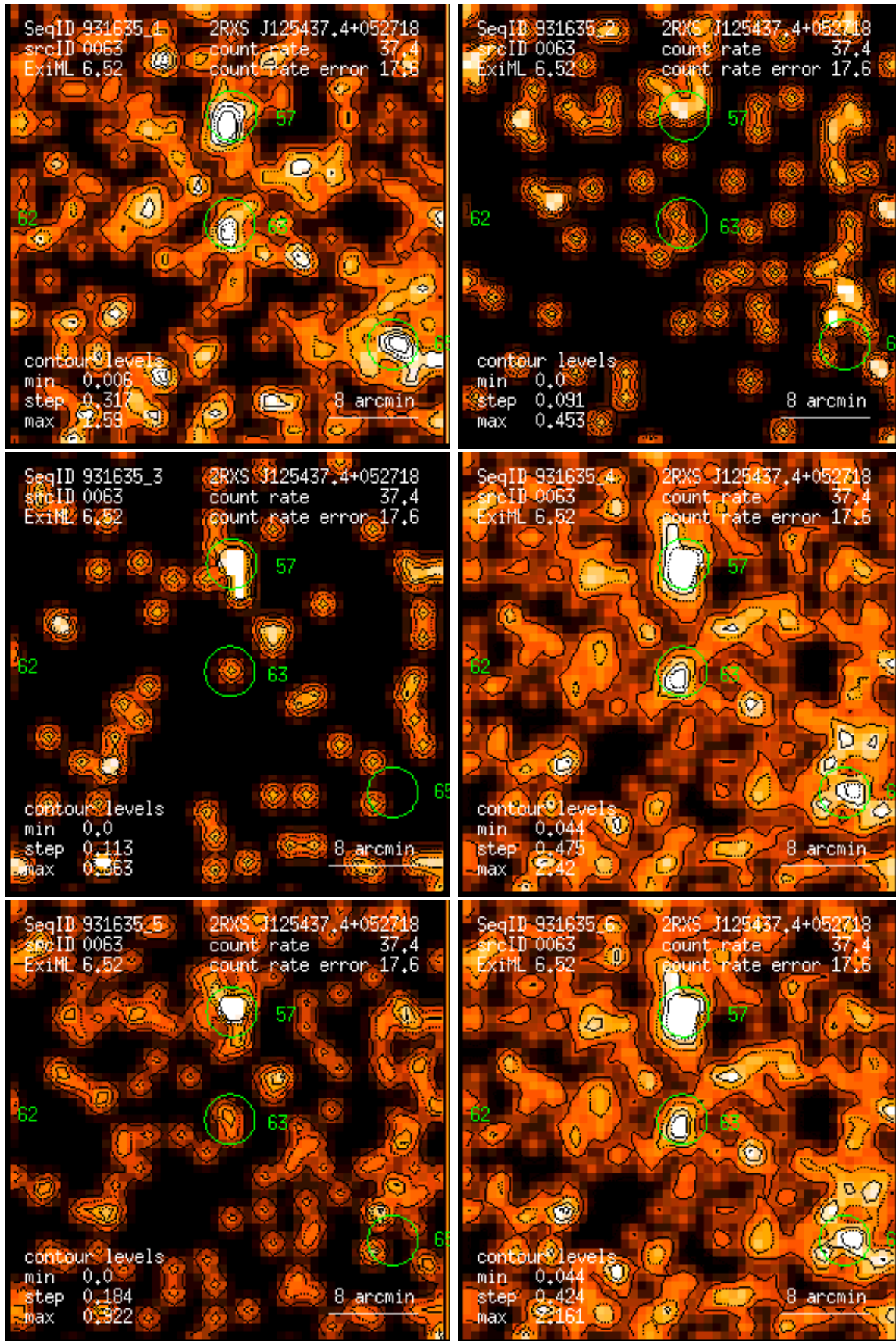
Figure 63: RASS 931635: detection 0063: band rate images, Gaussian filter: (1) PSPC channels 11 – 41, (2) 52 – 90, (3) 91 – 201, (4) 11 – 235, (5) 52 – 201, (6) 11 – 201. Broad band rates in counts/ks. Band rate contour levels in counts/ks/arcmin 2 .
