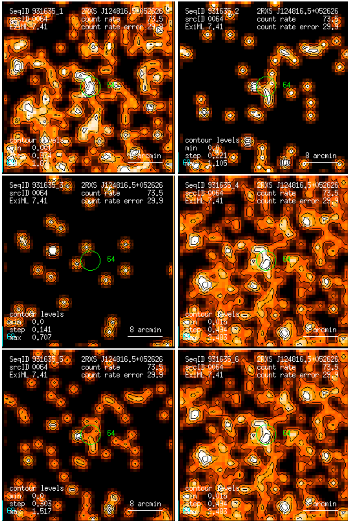
Figure 64: RASS 931635: detection 0064: band rate images, Gaussian filter: (1) PSPC channels 11 – 41, (2) 52 – 90, (3) 91 – 201, (4) 11 – 235, (5) 52 – 201, (6) 11 – 201. Broad band rates in counts/ks. Band rate contour levels in counts/ks/arcmin 2 .
