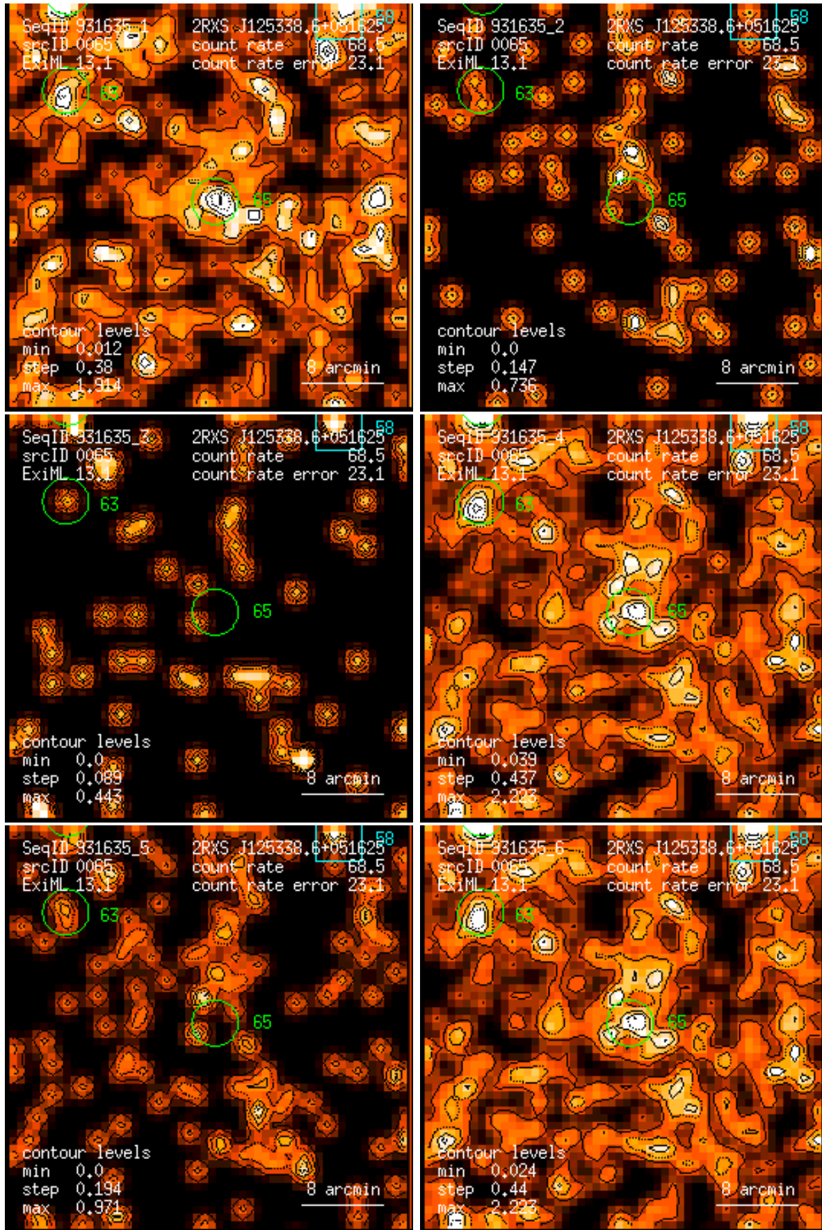
Figure 65: RASS 931635: detection 0065: band rate images, Gaussian filter: (1) PSPC channels 11 – 41, (2) 52 – 90, (3) 91 – 201, (4) 11 – 235, (5) 52 – 201, (6) 11 – 201. Broad band rates in counts/ks. Band rate contour levels in counts/ks/arcmin 2 .
