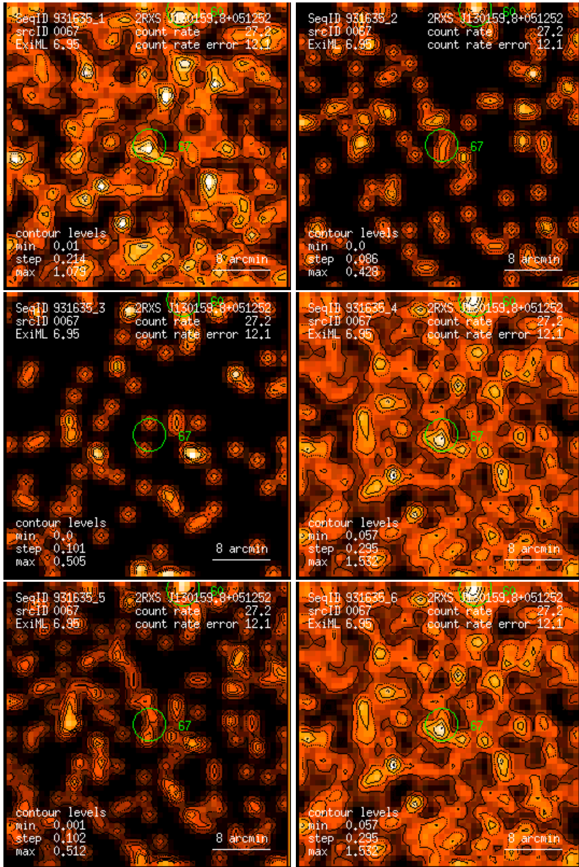
Figure 67: RASS 931635: detection 0067: band rate images, Gaussian filter: (1) PSPC channels 11 – 41, (2) 52 – 90, (3) 91 – 201, (4) 11 – 235, (5) 52 – 201, (6) 11 – 201. Broad band rates in counts/ks. Band rate contour levels in counts/ks/arcmin 2 .
