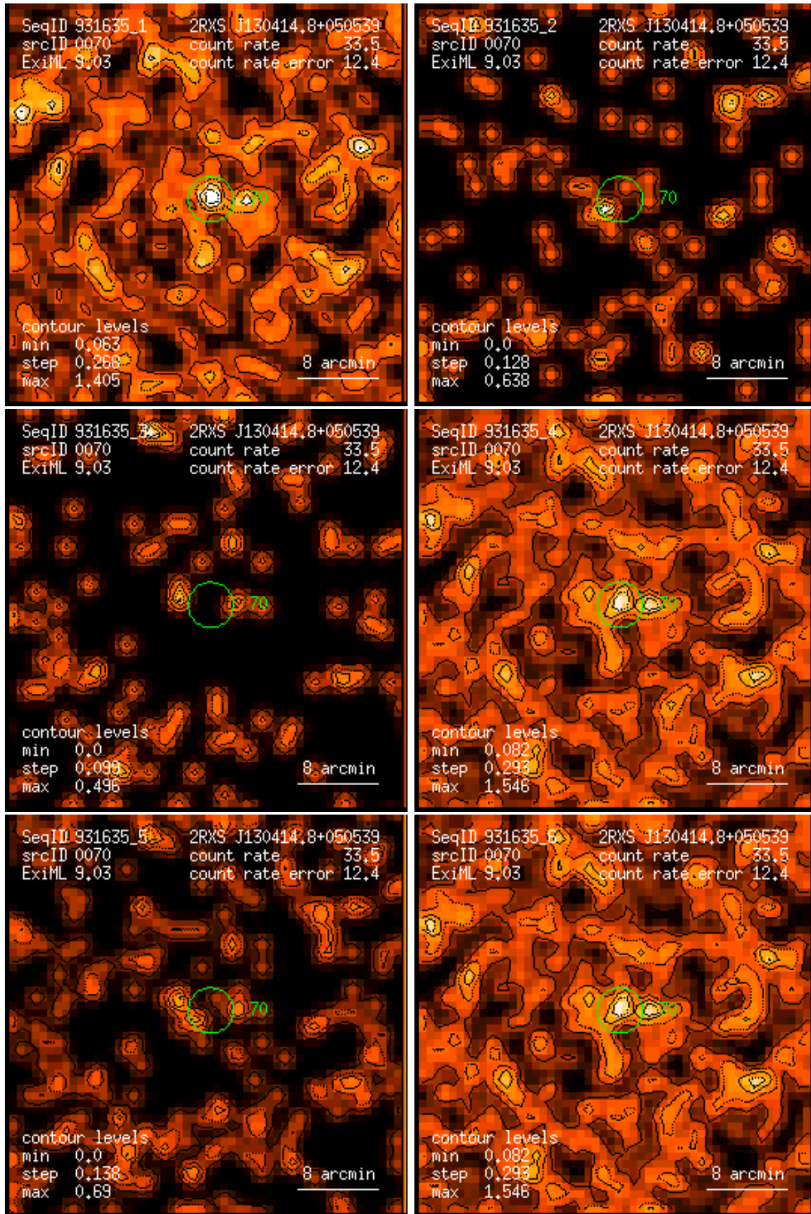
Figure 70: RASS 931635: detection 0070: band rate images, Gaussian filter: (1) PSPC channels 11 – 41, (2) 52 – 90, (3) 91 – 201, (4) 11 – 235, (5) 52 – 201, (6) 11 – 201. Broad band rates in counts/ks. Band rate contour levels in counts/ks/arcmin 2 .
