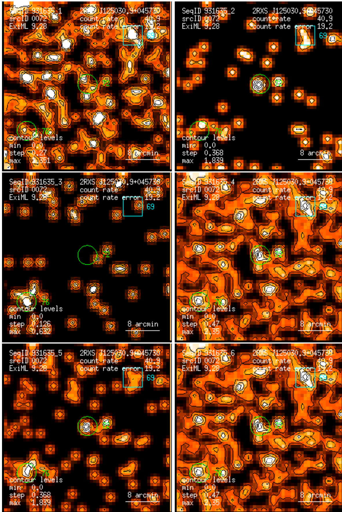
Figure 72: RASS 931635: detection 0072: band rate images, Gaussian filter: (1) PSPC channels 11 – 41, (2) 52 – 90, (3) 91 – 201, (4) 11 – 235, (5) 52 – 201, (6) 11 – 201. Broad band rates in counts/ks. Band rate contour levels in counts/ks/arcmin 2 .
