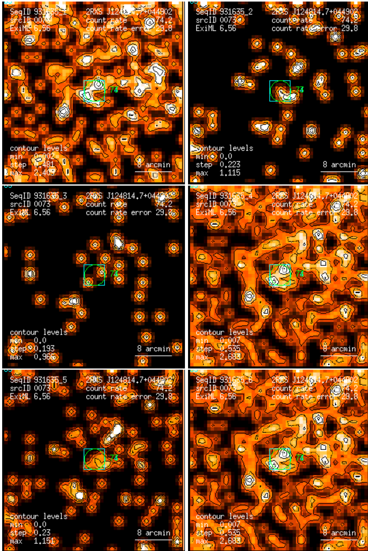
Figure 73: RASS 931635: detection 0073: band rate images, Gaussian filter: (1) PSPC channels 11 – 41, (2) 52 – 90, (3) 91 – 201, (4) 11 – 235, (5) 52 – 201, (6) 11 – 201. Broad band rates in counts/ks. Band rate contour levels in counts/ks/arcmin 2 .
